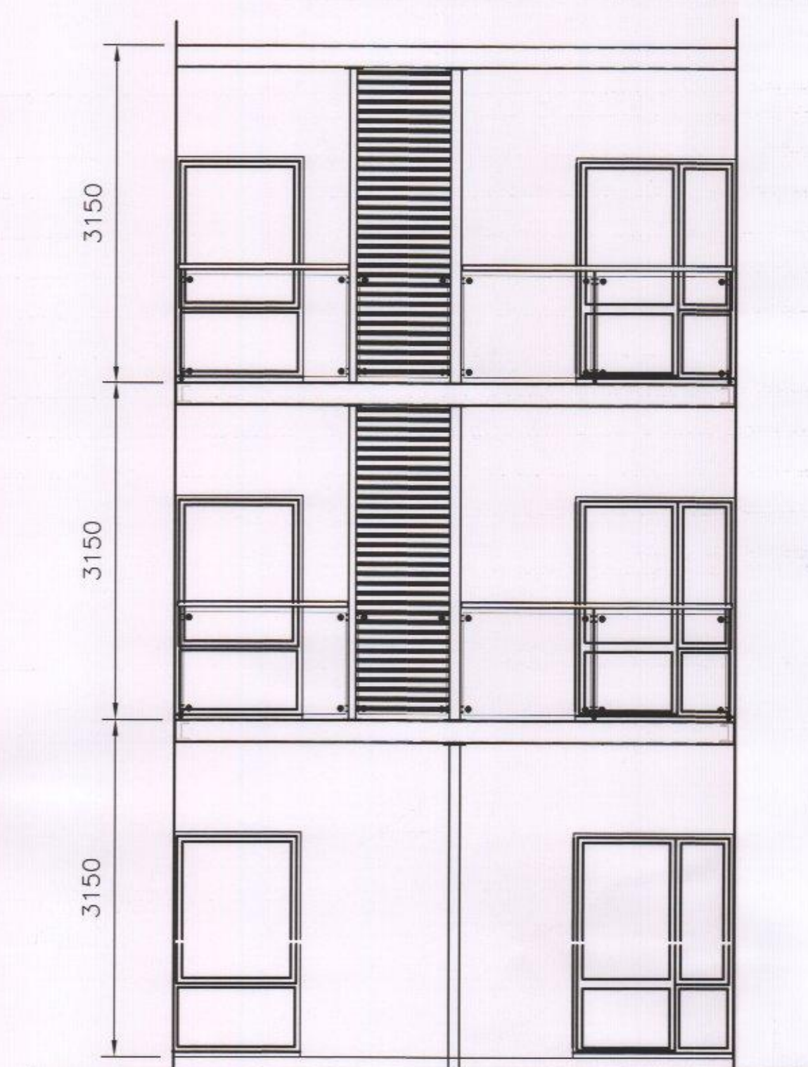
ELEVATION - TYPICAL BAY Scale 1:50
