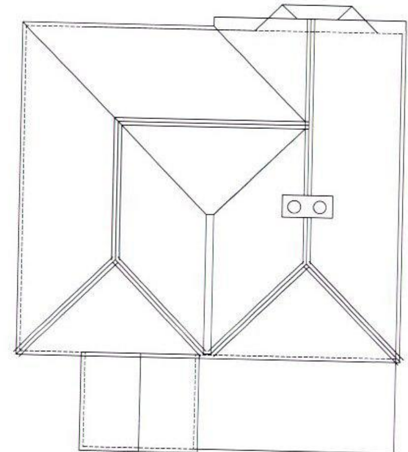
Roof Floor Plan 1:100
