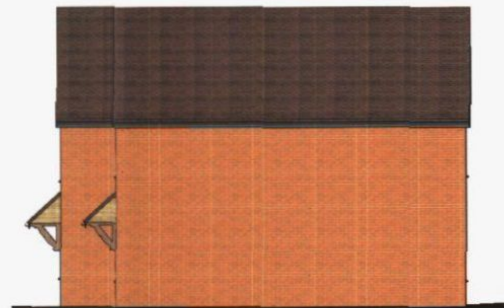
Type 12- Plots 51,52 Right Elevation 1 : 100
