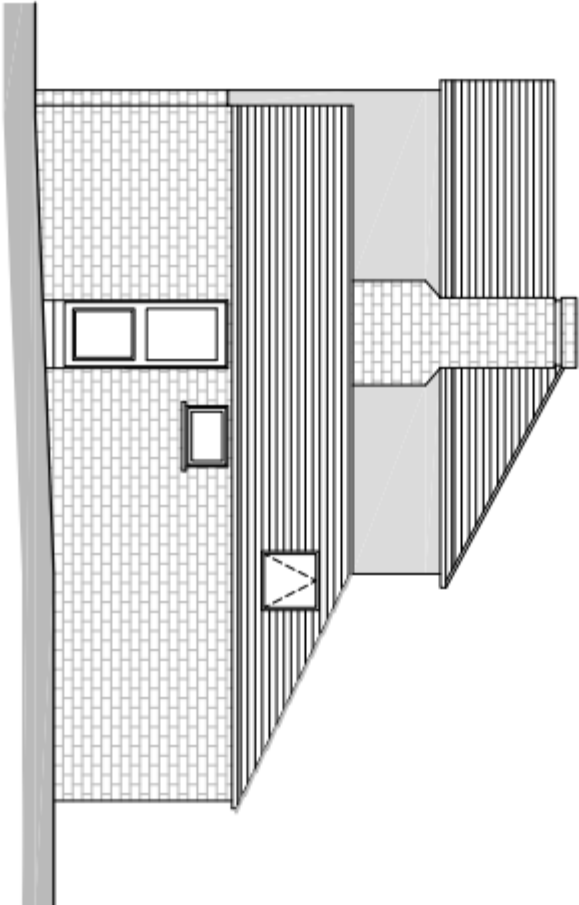
SOUTH ELEVATION 1 : 100
