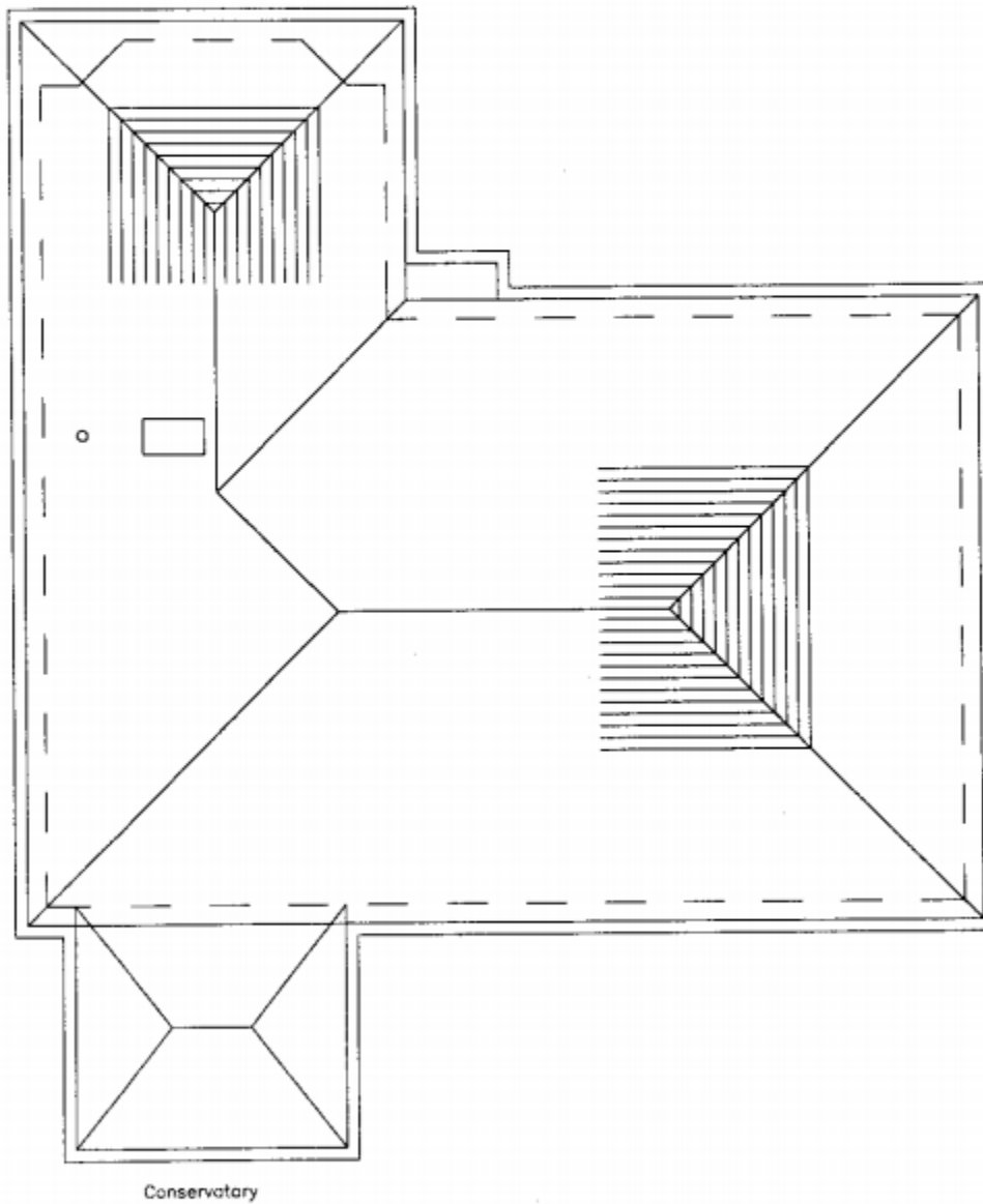
ROOF PLAN
