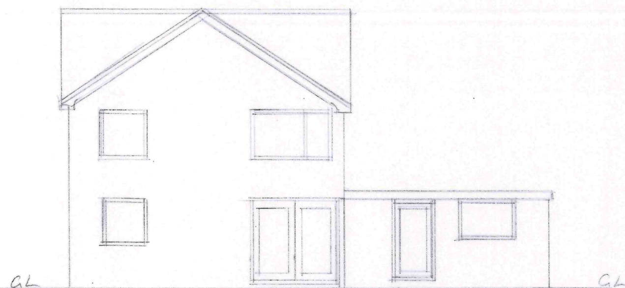
EXG REAR ELEVATION
