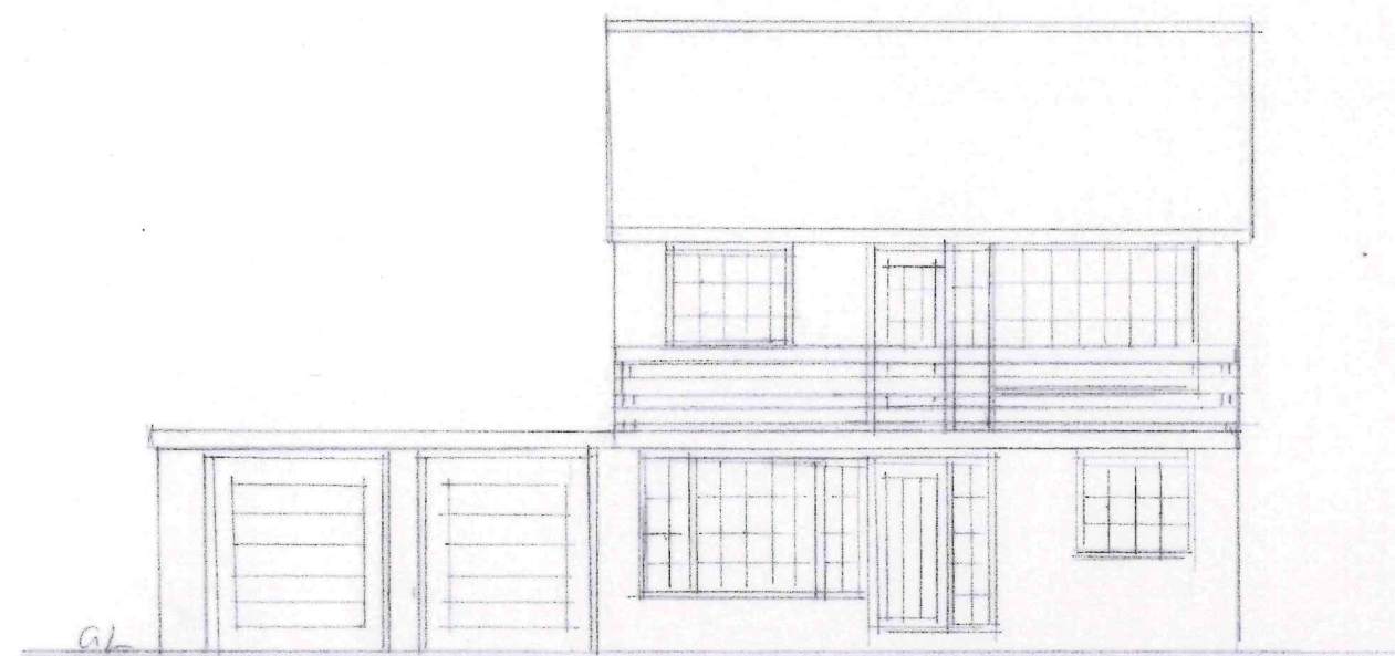
EXG FRONT ELEVATION
