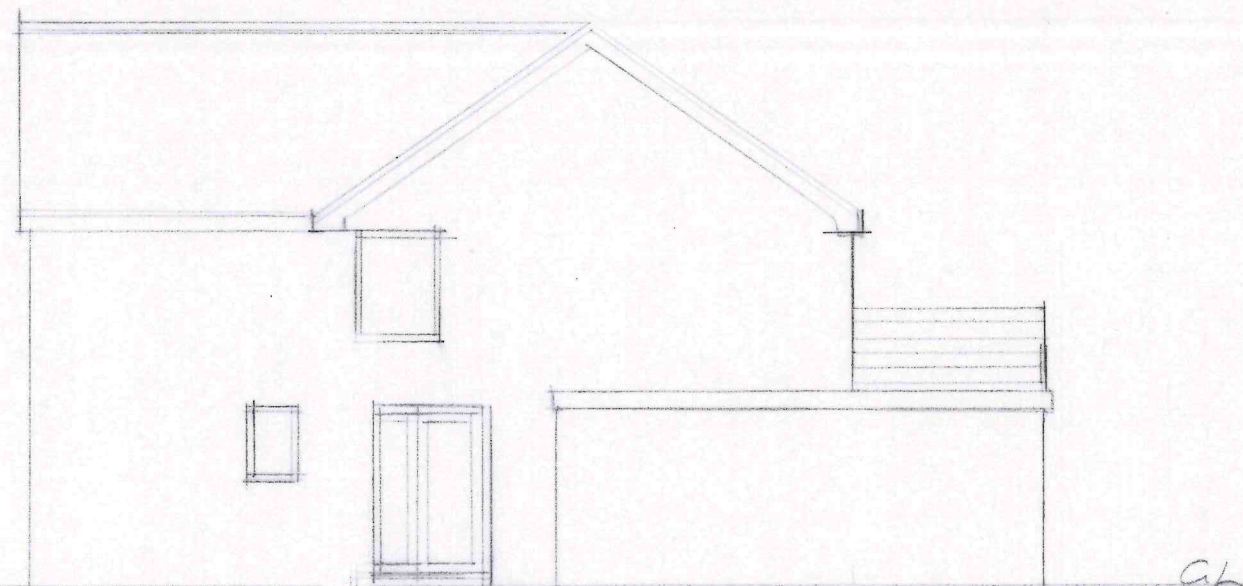
EXG SIDE ELEVATION
