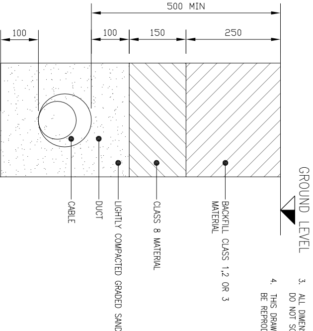
BURIED IN DUCT
