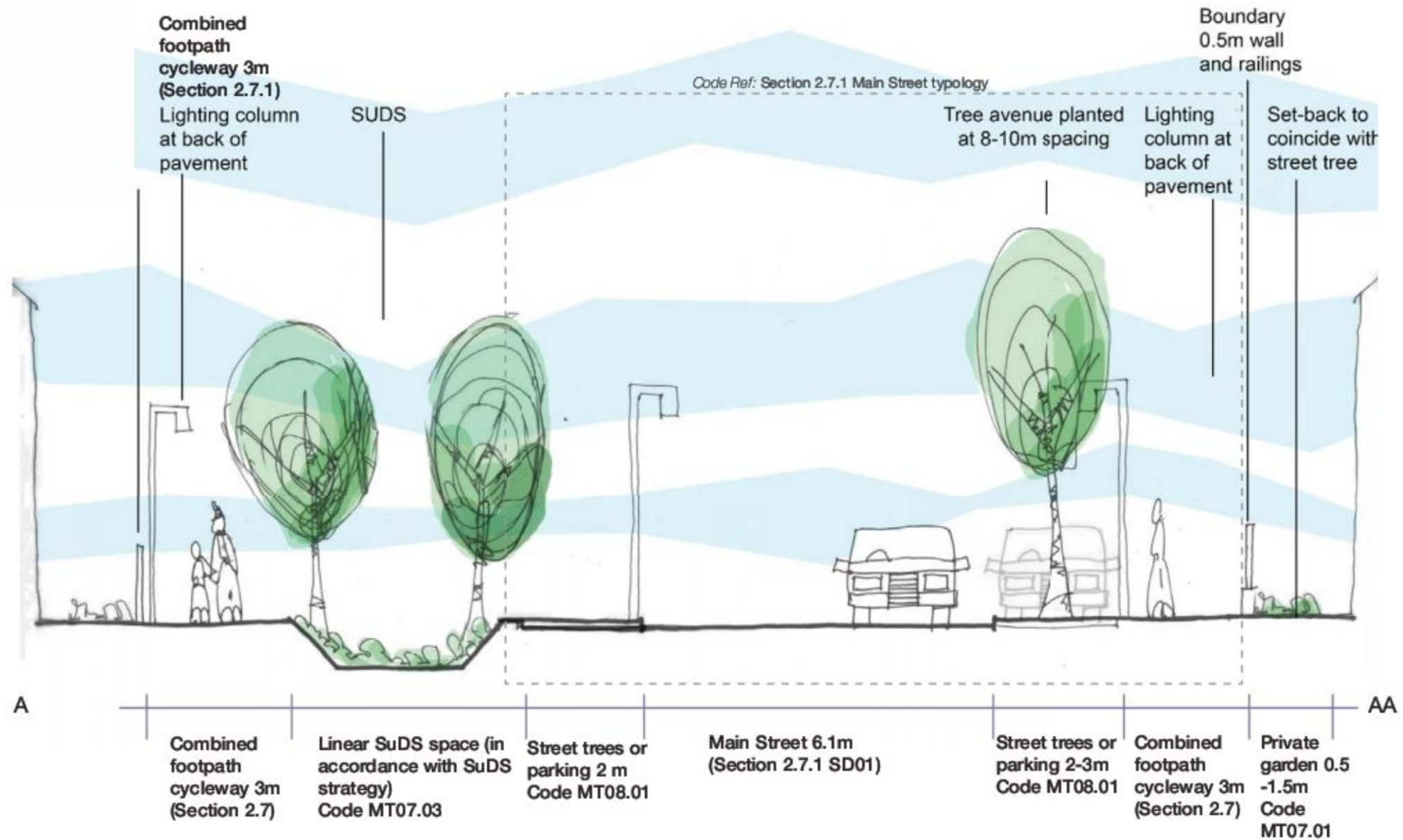
MT4 Section
