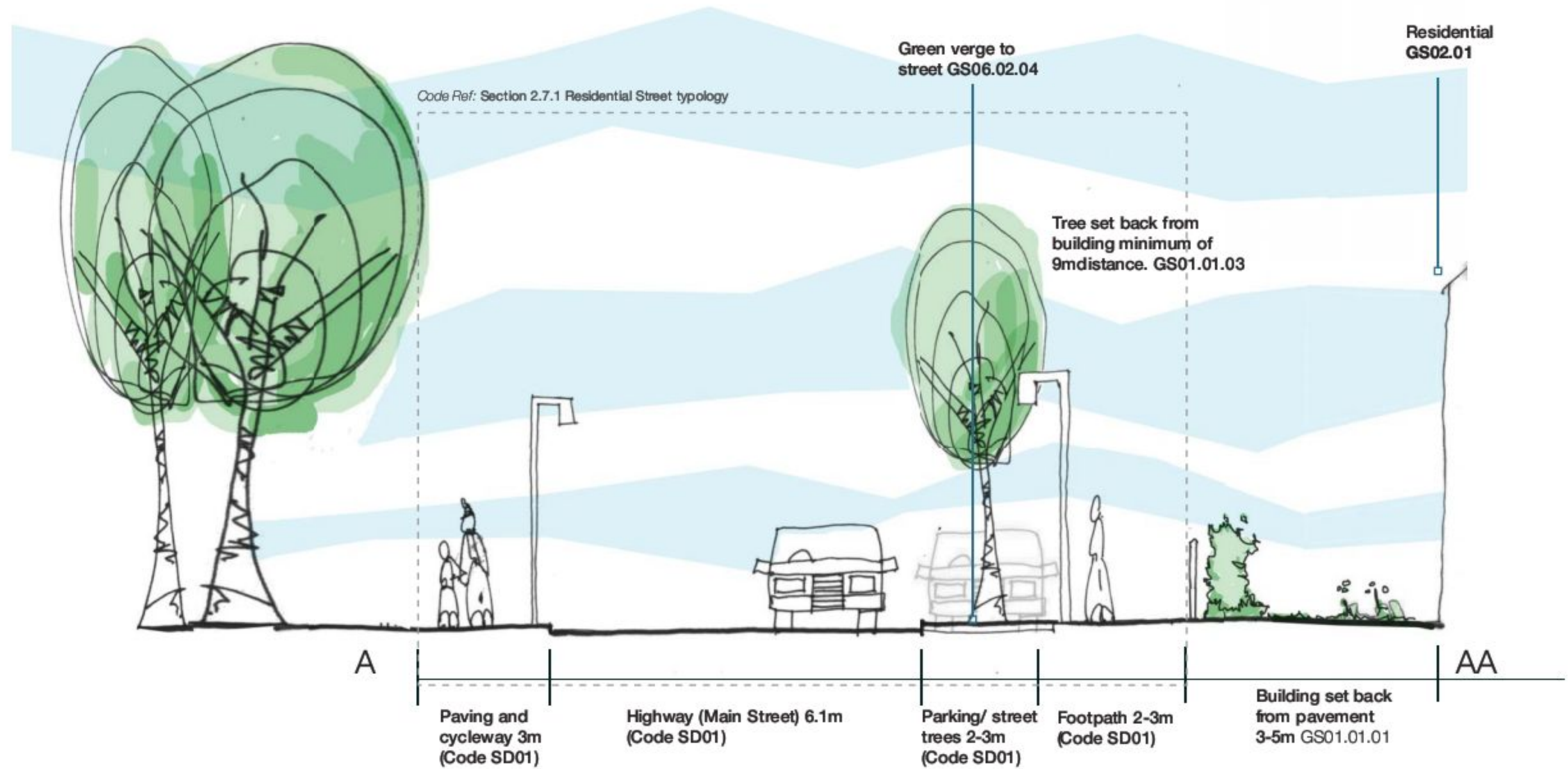
GS3 Section
