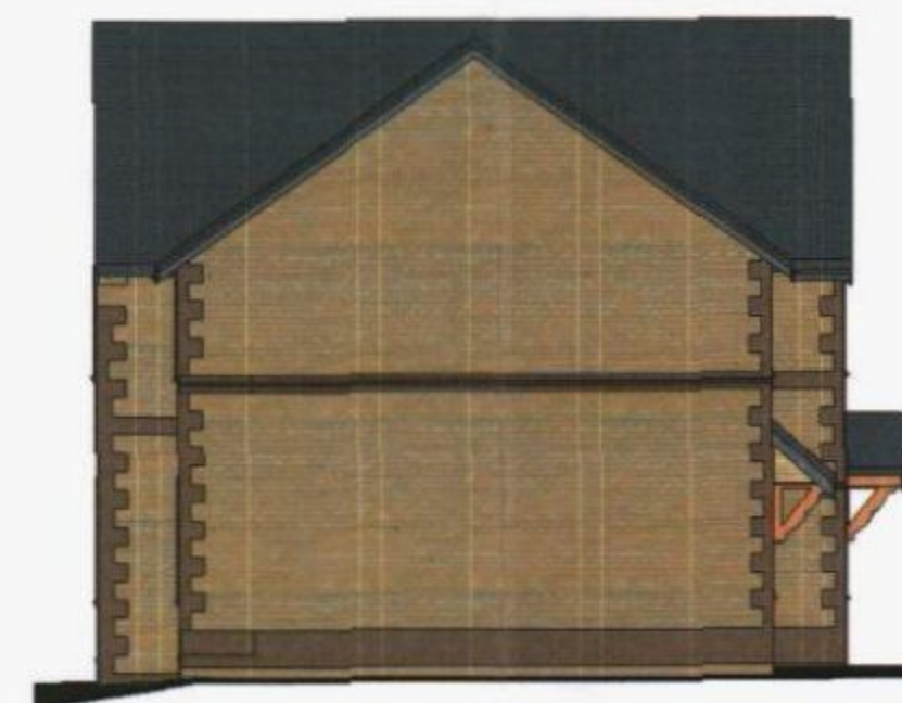
Type 5- Plots 11,12 Right Elevation 1:100
