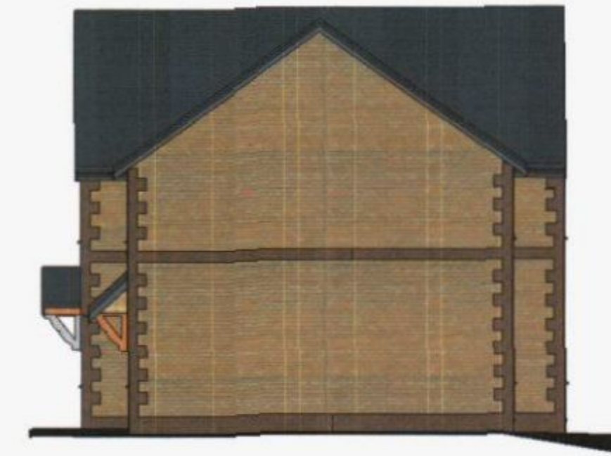
Type 6- Plots 13,14,57,58 Right elevation 1:100
