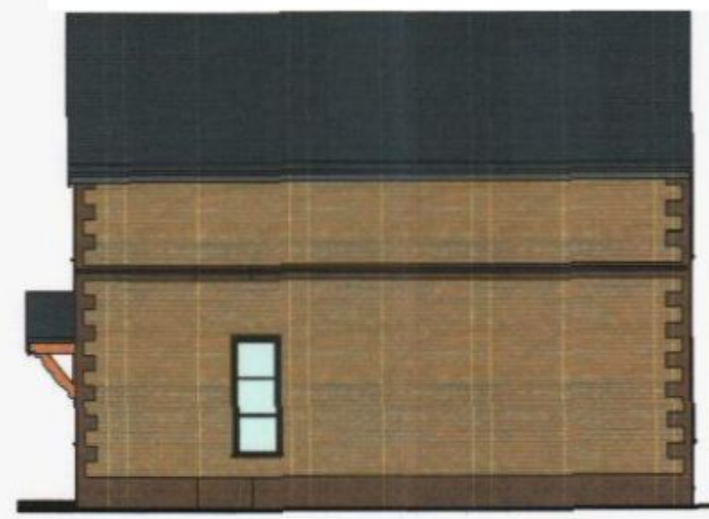
Type 5- Plots 11,12 Right Elevation 1:100
