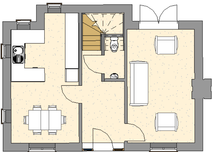
Type 20- Plots 17 Ground Floor 1 : 100
