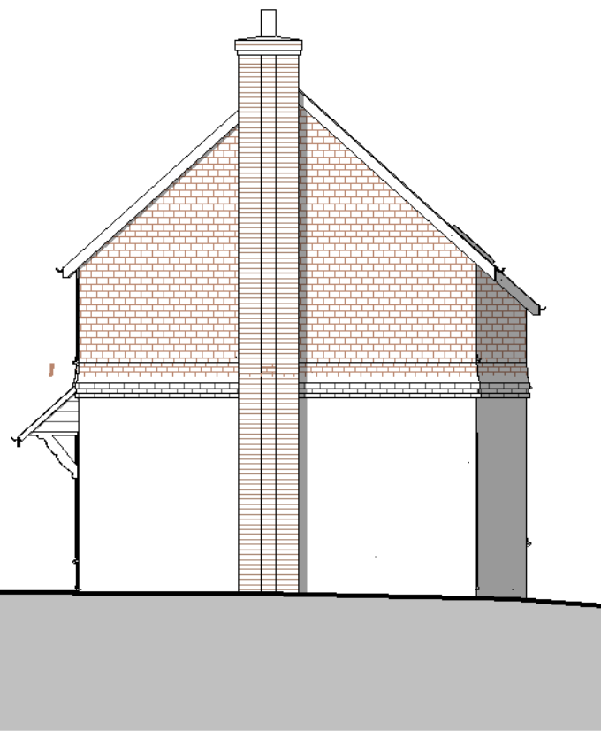
Type 20- Plot 17 Rear Elevation 1 : 100
