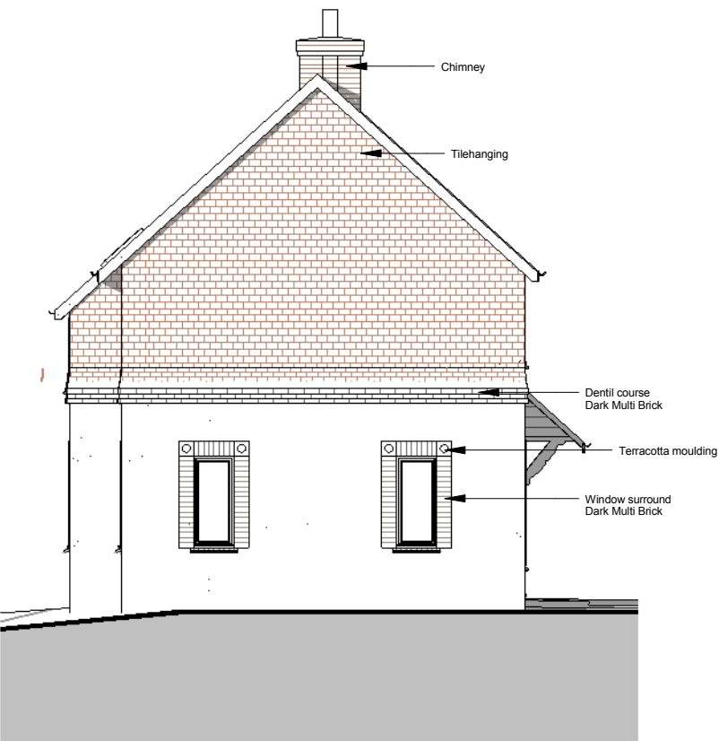
Type 20- Plot 17 Front Elevation 1 : 100
