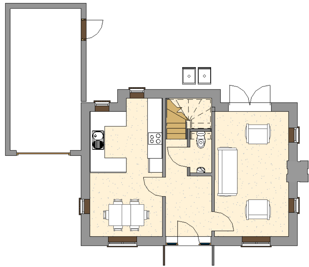
Type 21- Plot 42 Ground Floor 1 : 100
