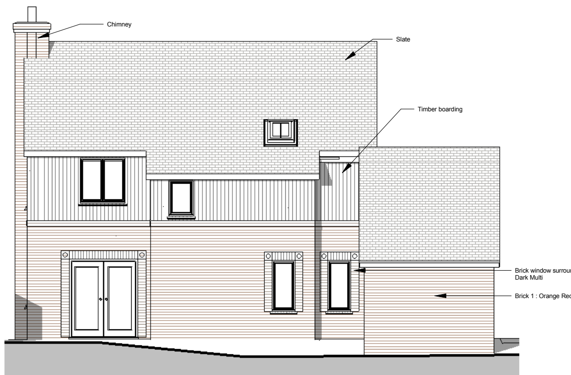
Type 21- Plot 42 Rear Elevation 1 : 100
