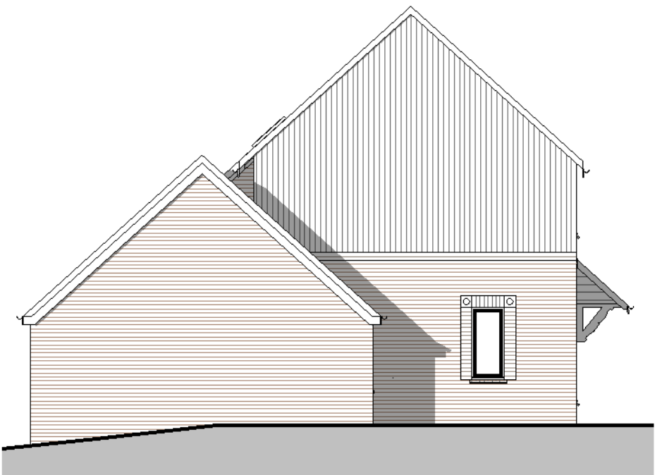
Type 21- Plot 42 Left Elevation 1 : 100
