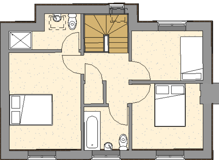
Type 20- Plots 17 First Floor 1 : 100
