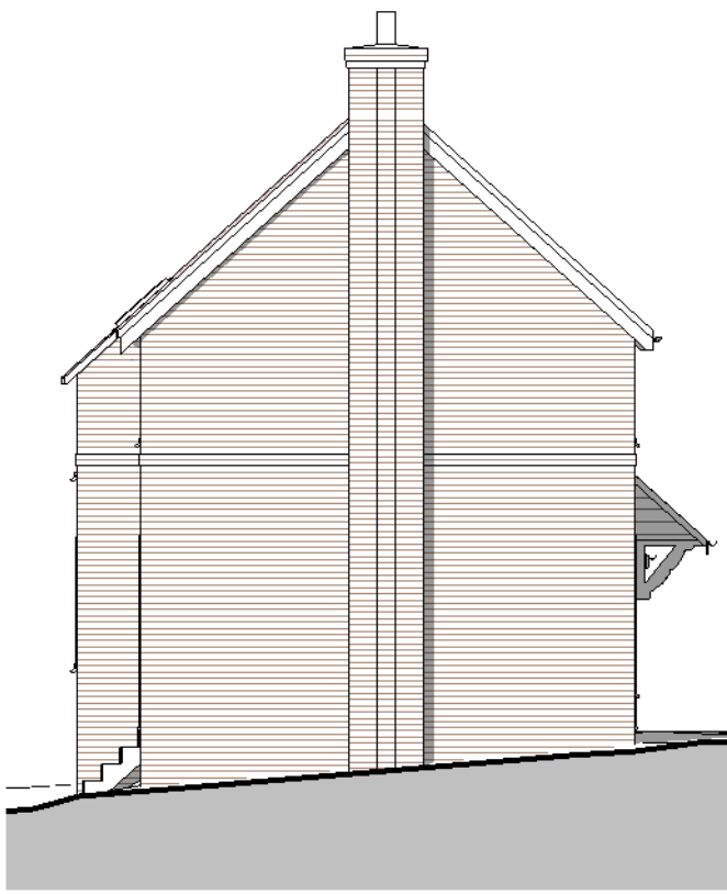
Type 19- Plot 16 Left Elevation 1 : 100
