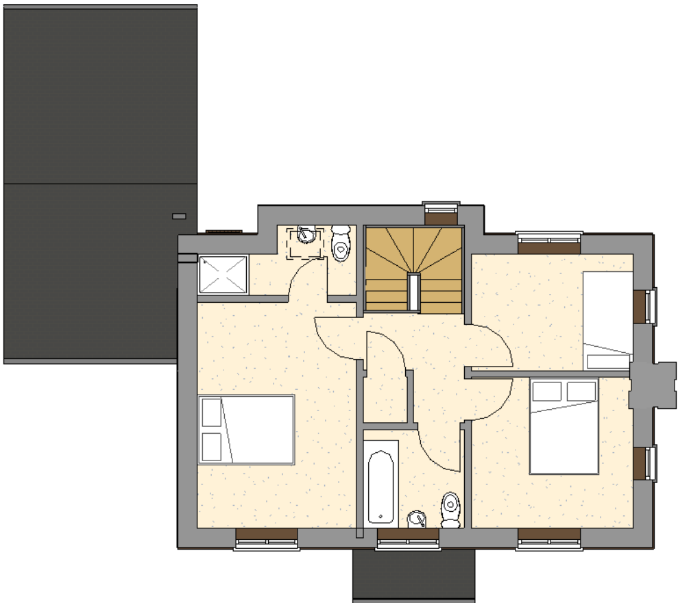
Type 21- Plot 42 First Floor 1 : 100
