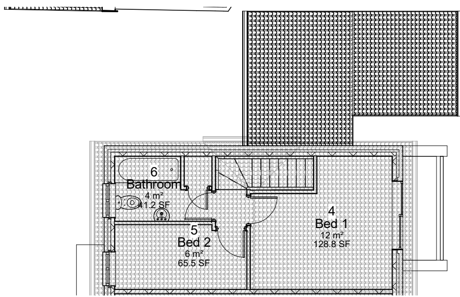
2 First Floor Plan 1 : 100
