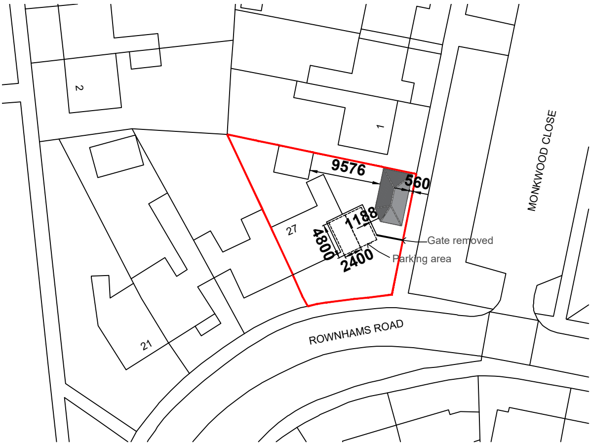
BLOCK PLAN 1:500
