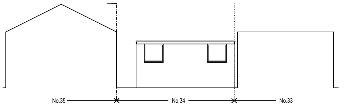
FRONT ELEVATION 1:100 [East / Garden facing]
