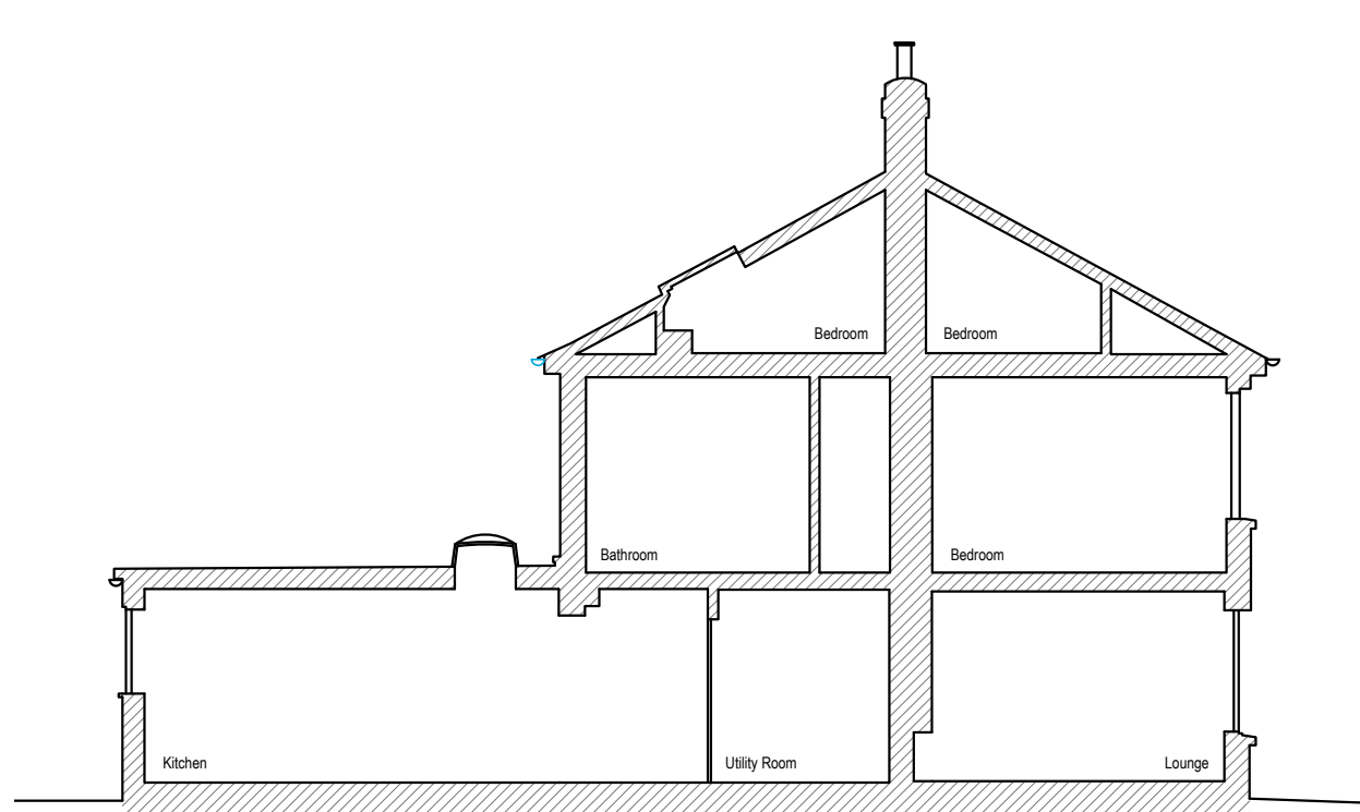
SECTION 1:100
