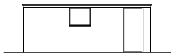
SIDE ELEVATION 1:100 [North]
