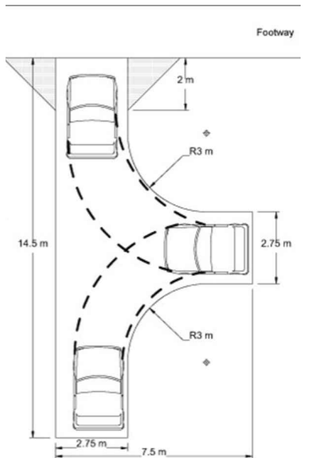
TURNING CIRCLE DIAGRAM
