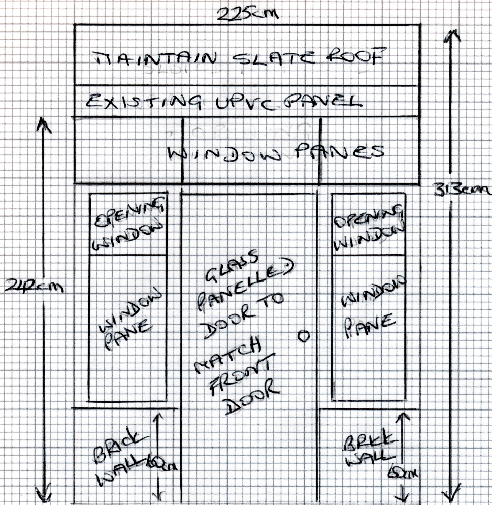
PROPOSED PORCH FRONT ELEVATION
