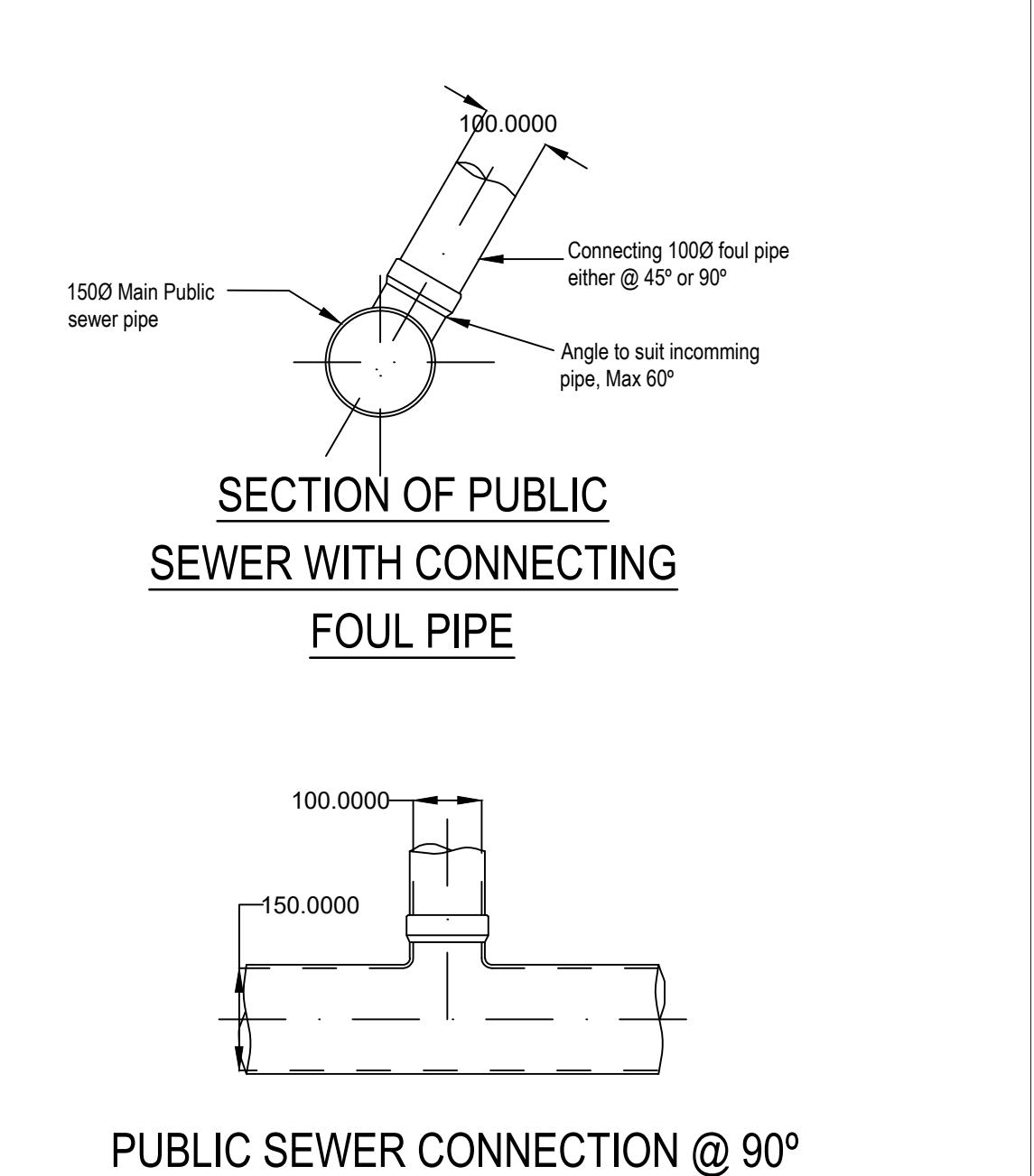
PUBLIC SEWER CONNECTION @ 90°
