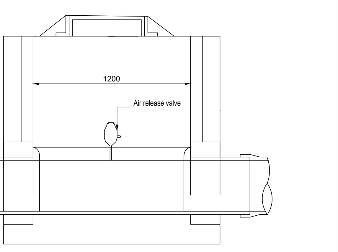
AIR RELEASE MANHOLE DETAIL
