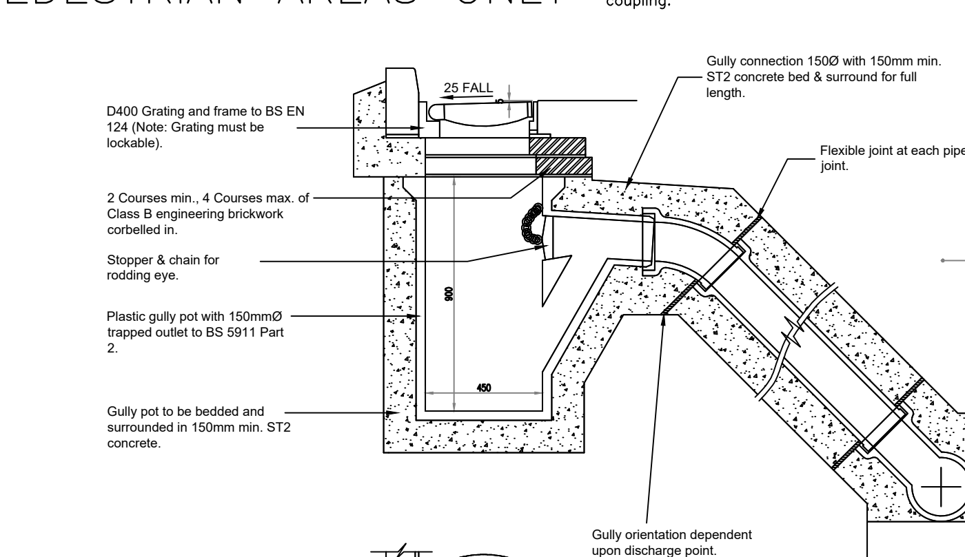
RODDING EYE PEDESTRIAN AREAS ONLY
