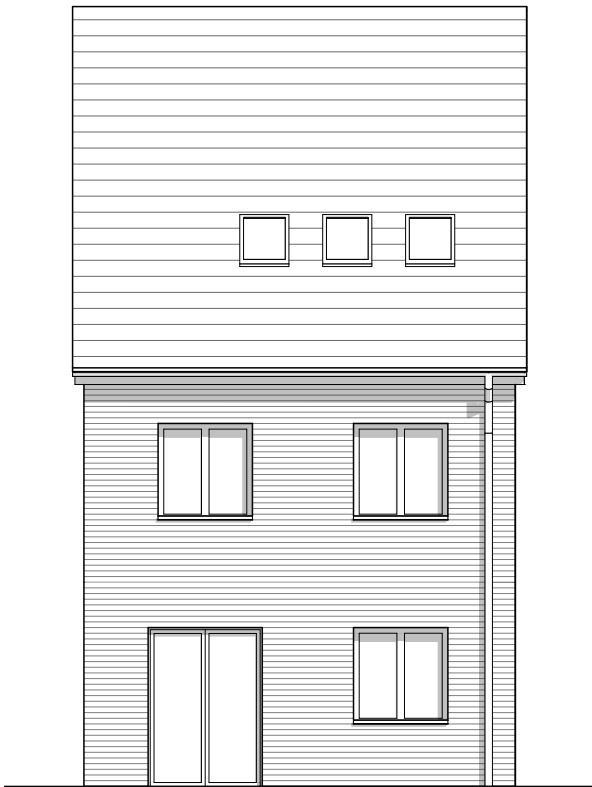
Rear Elevation
