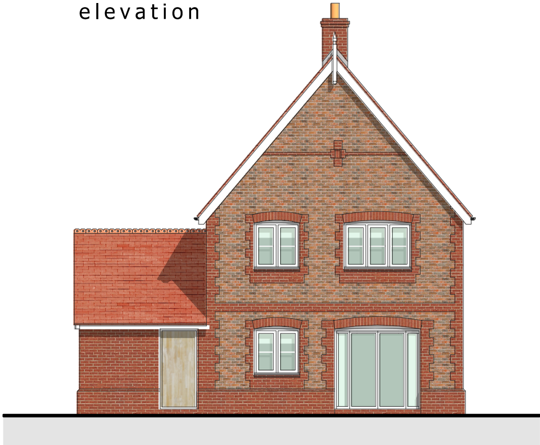
REAR elevation
