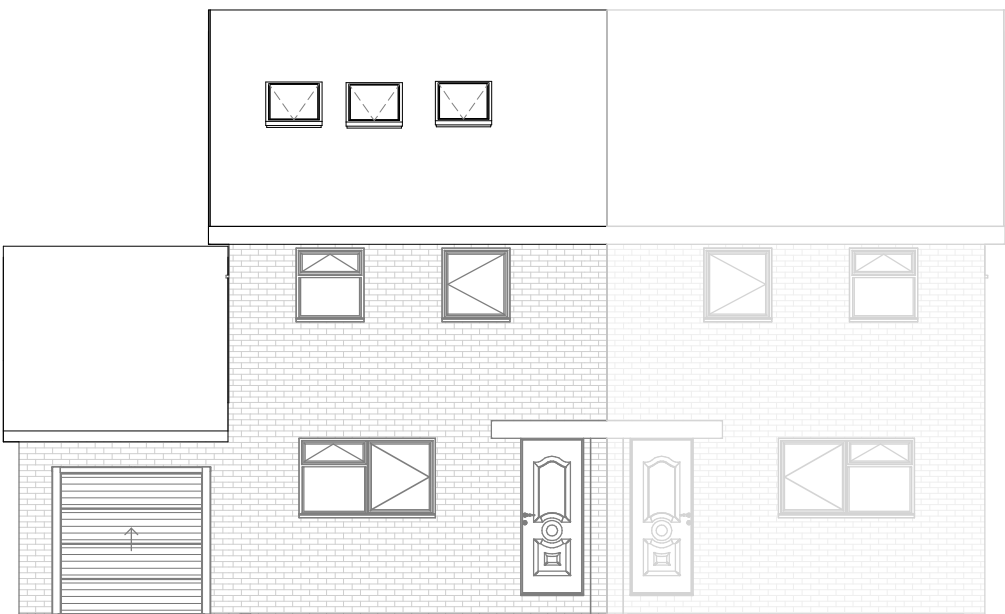
Proposed Elevation-Front
