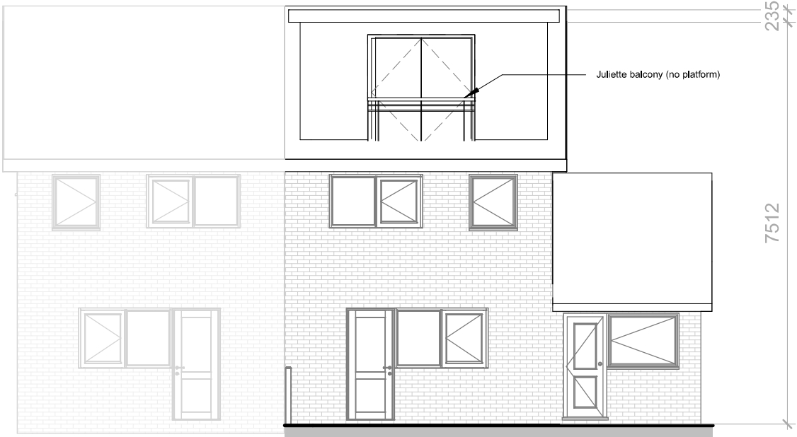
Proposed Elevation-Rear
