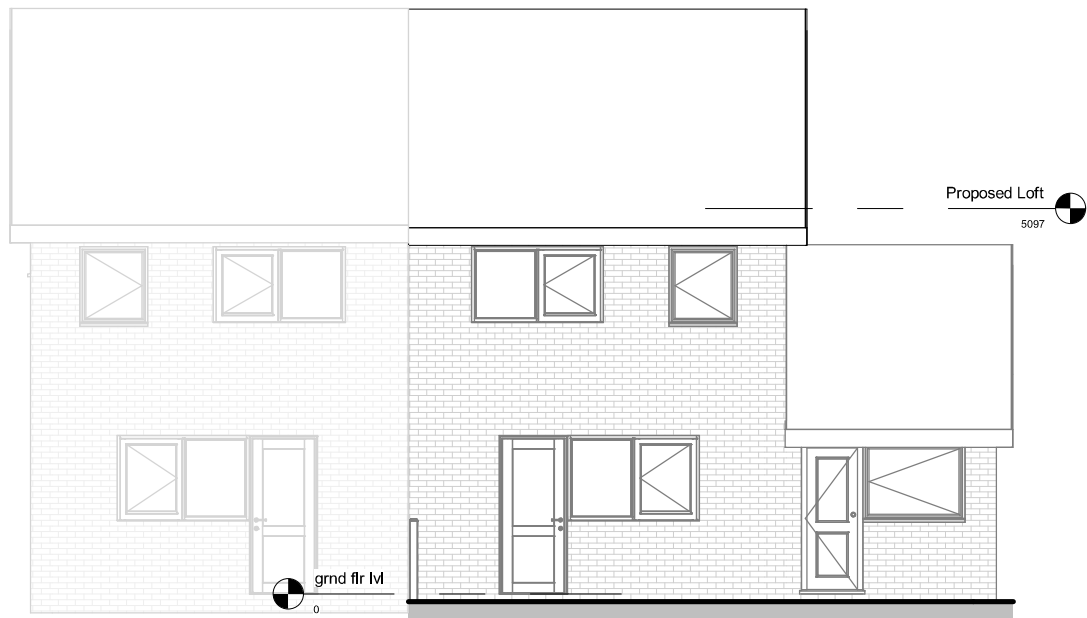
Existing Elevation-Rear
