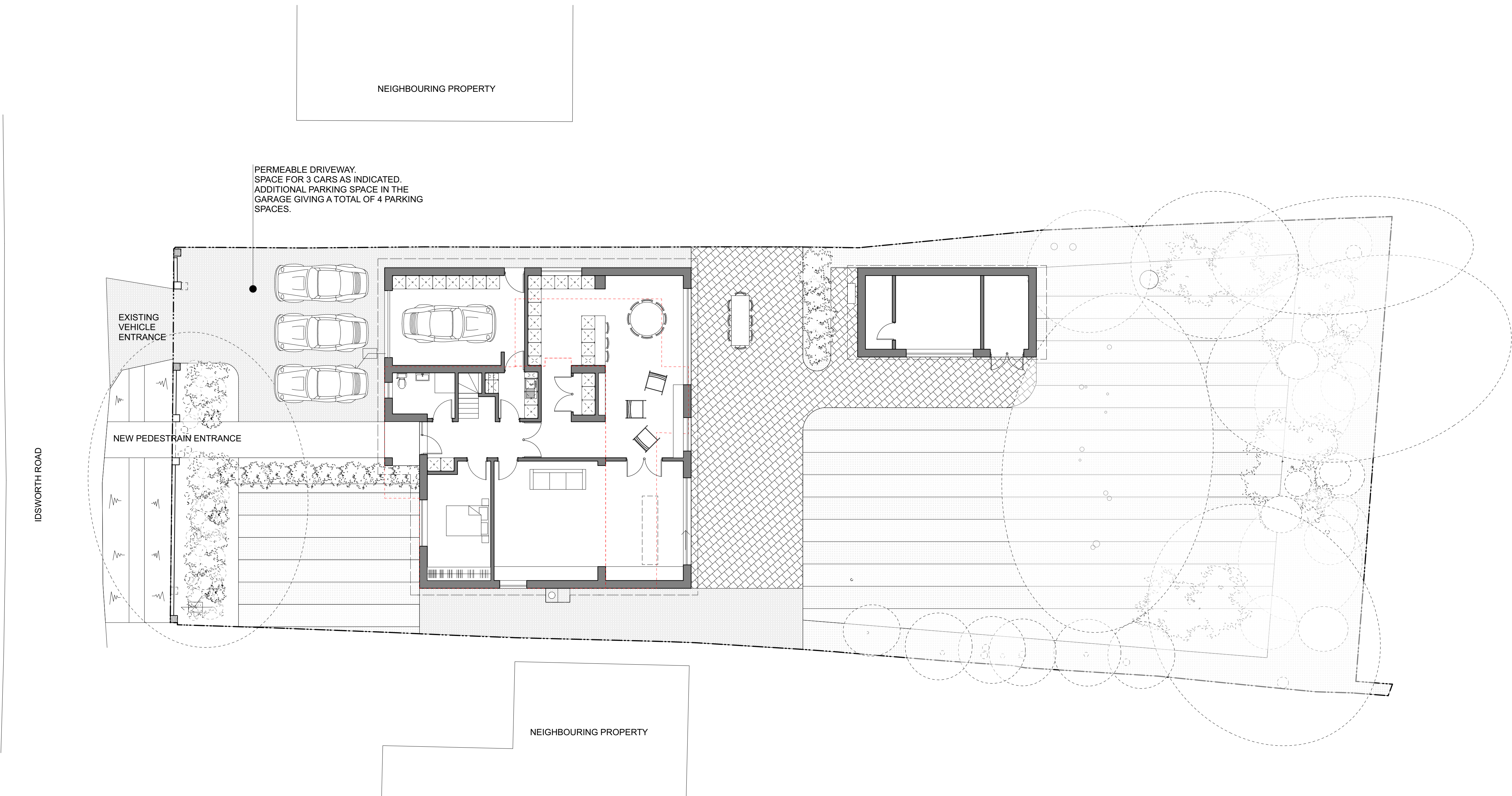
01 PROPOSED PARKING PLAN 1:100 0 1 2 3 4 5 M
