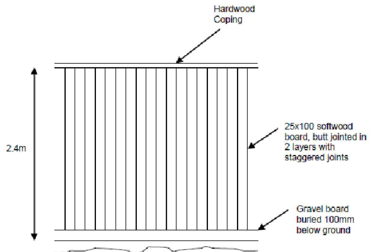
Acoustic Fence Elevation
