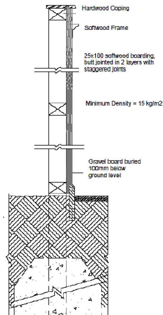
Acoustic Fence Cross Section
