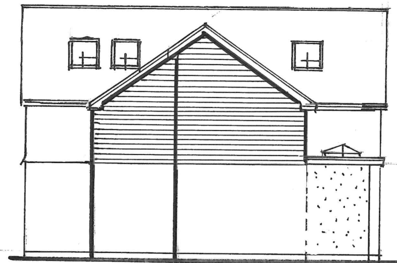
SIDE ELEVATION - PROPOSED
