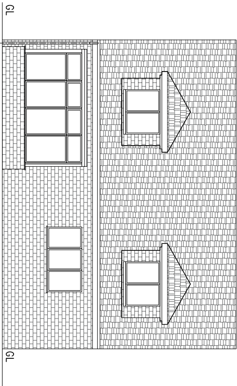
1 EXISTING REAR VIEW SCALE 1:100
