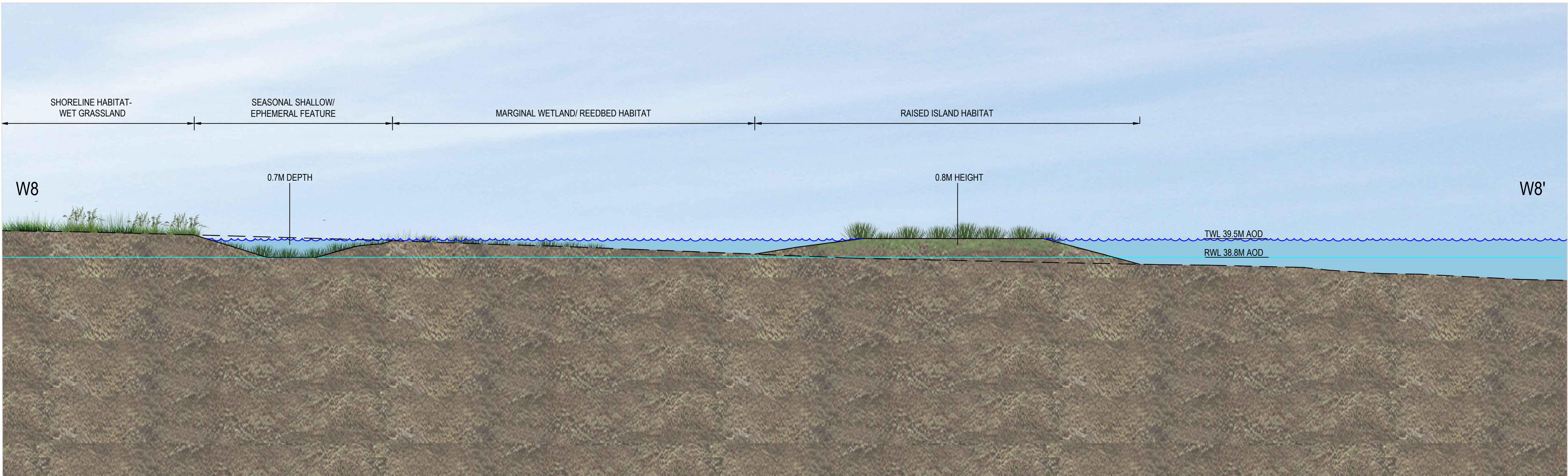
W8 - TYPICAL CROSS-SECTION THROUGH WETLAND ISLANDS AND EPHEMERAL FEATURES SCALE 1:100
