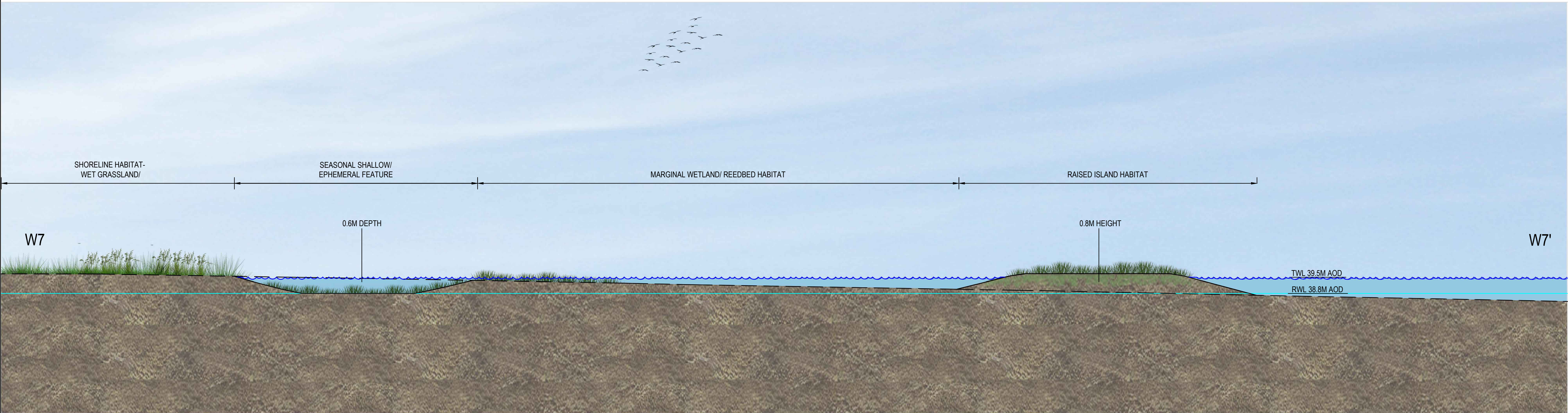
W7 - TYPICAL CROSS-SECTION THROUGH RAISED ISLANDS AND EPHEMERAL FEATURES SCALE 1:100
