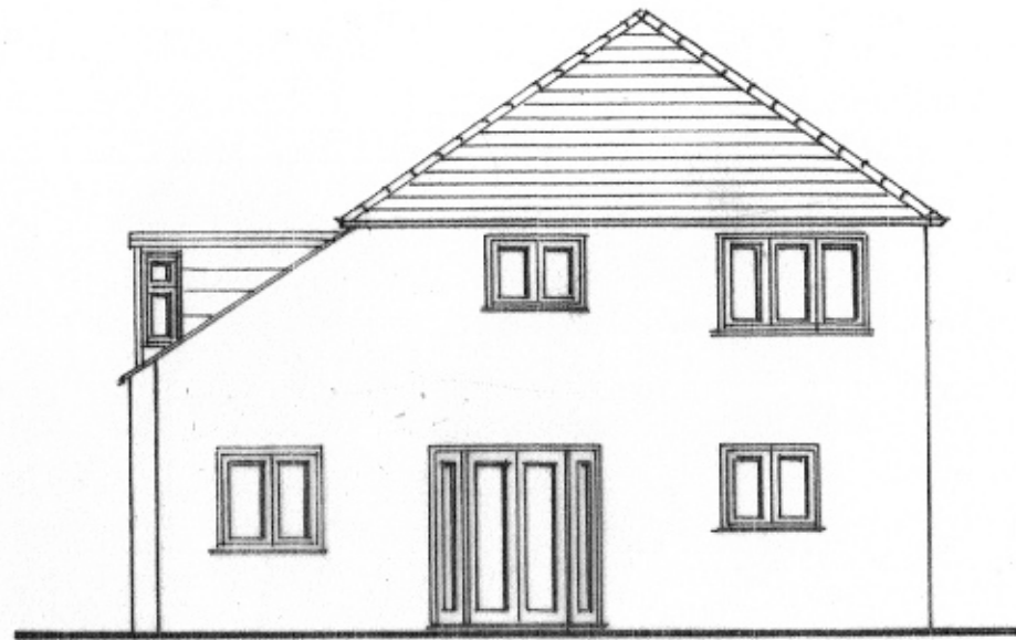
NORTH EAST ELEVATION as proposed
