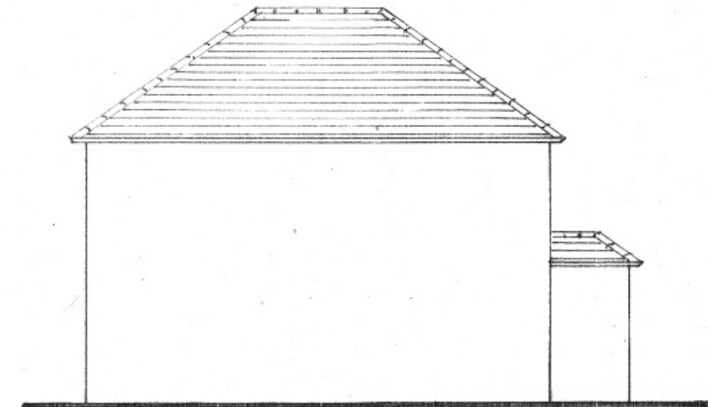
NORTH WEST ELEVATION as existing and proposed
