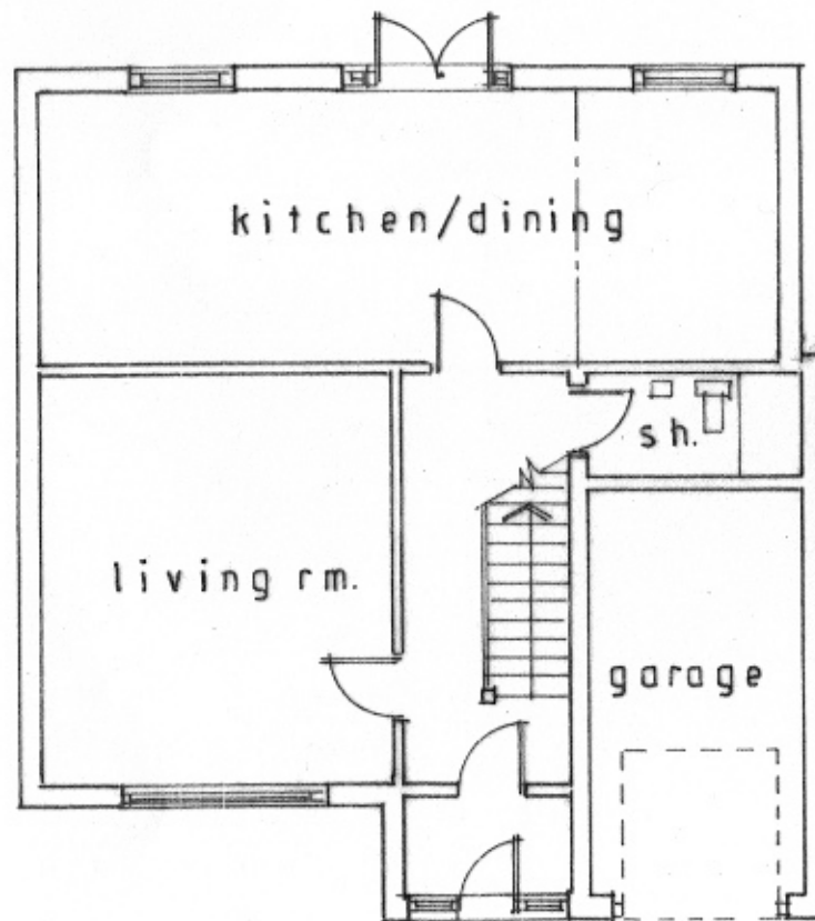
GROUND FLOOR PLAN as proposed
