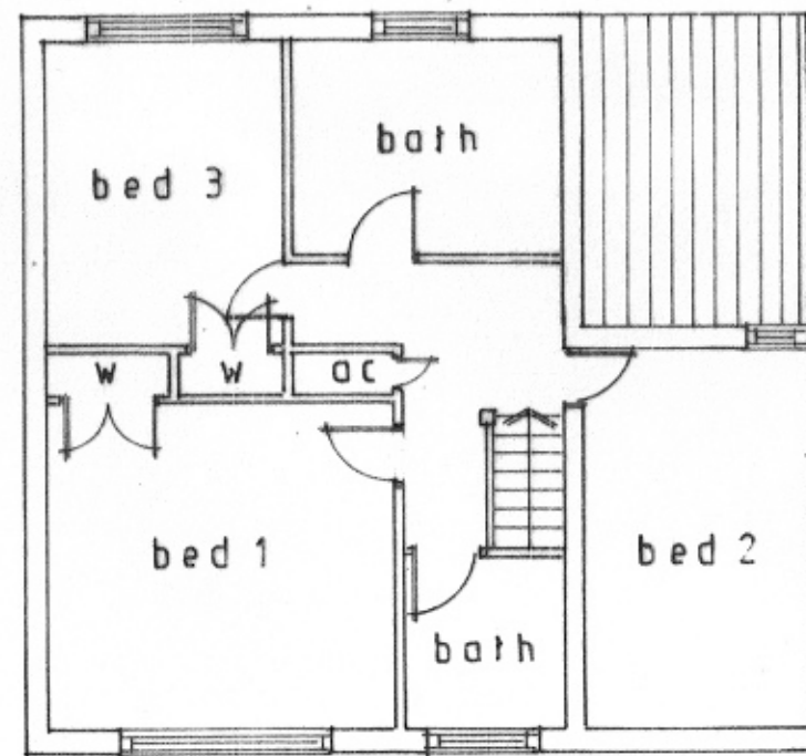
FIRST FLOOR PLAN 1:100 as proposed
