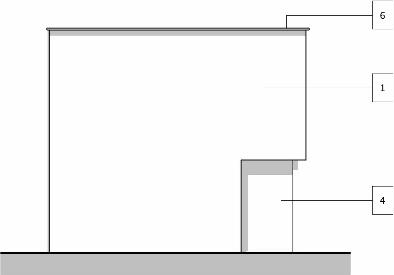
2 East Elevation - 1 : 100
