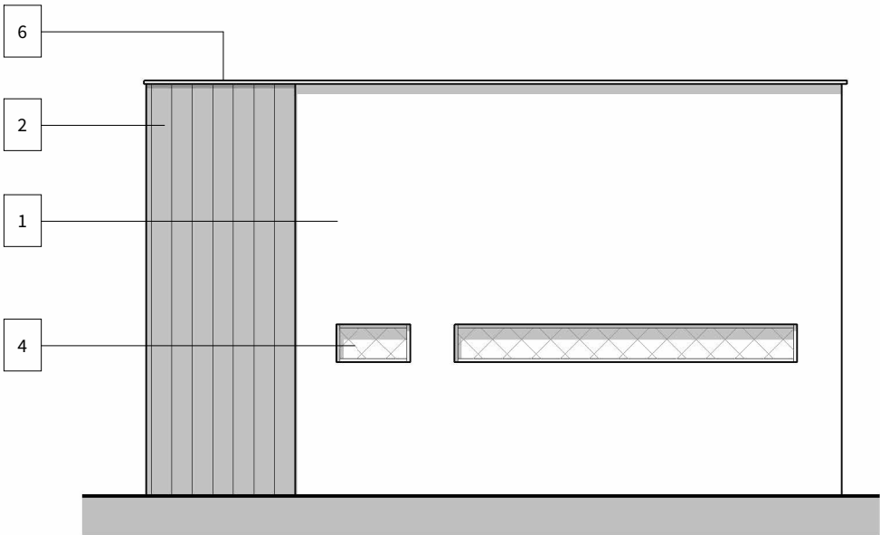
3 South Elevation - 1 : 100
