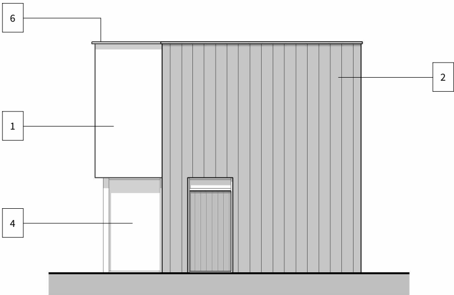
4 West Elevation - 1 : 100
