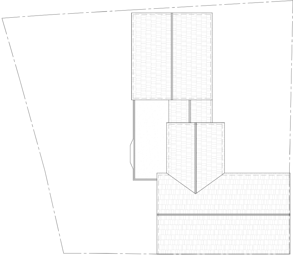
Existing Roof Plan Scale 1:50
