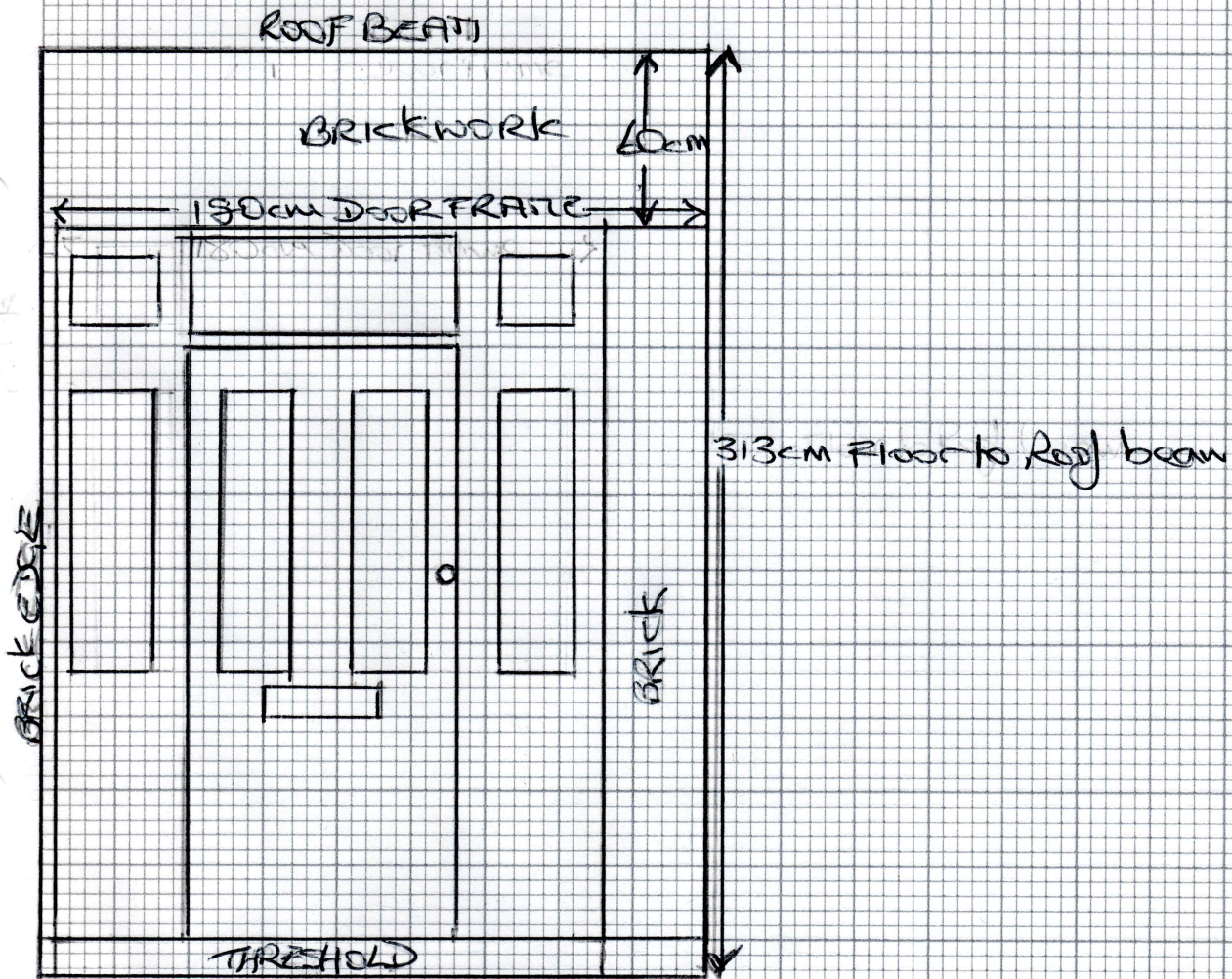
FRONT ELEVATION OF EXISTING DOOR
