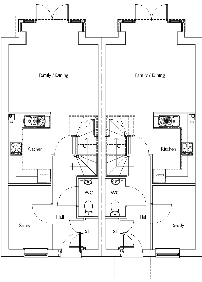
No. 31 GROUND FLOOR PLAN
