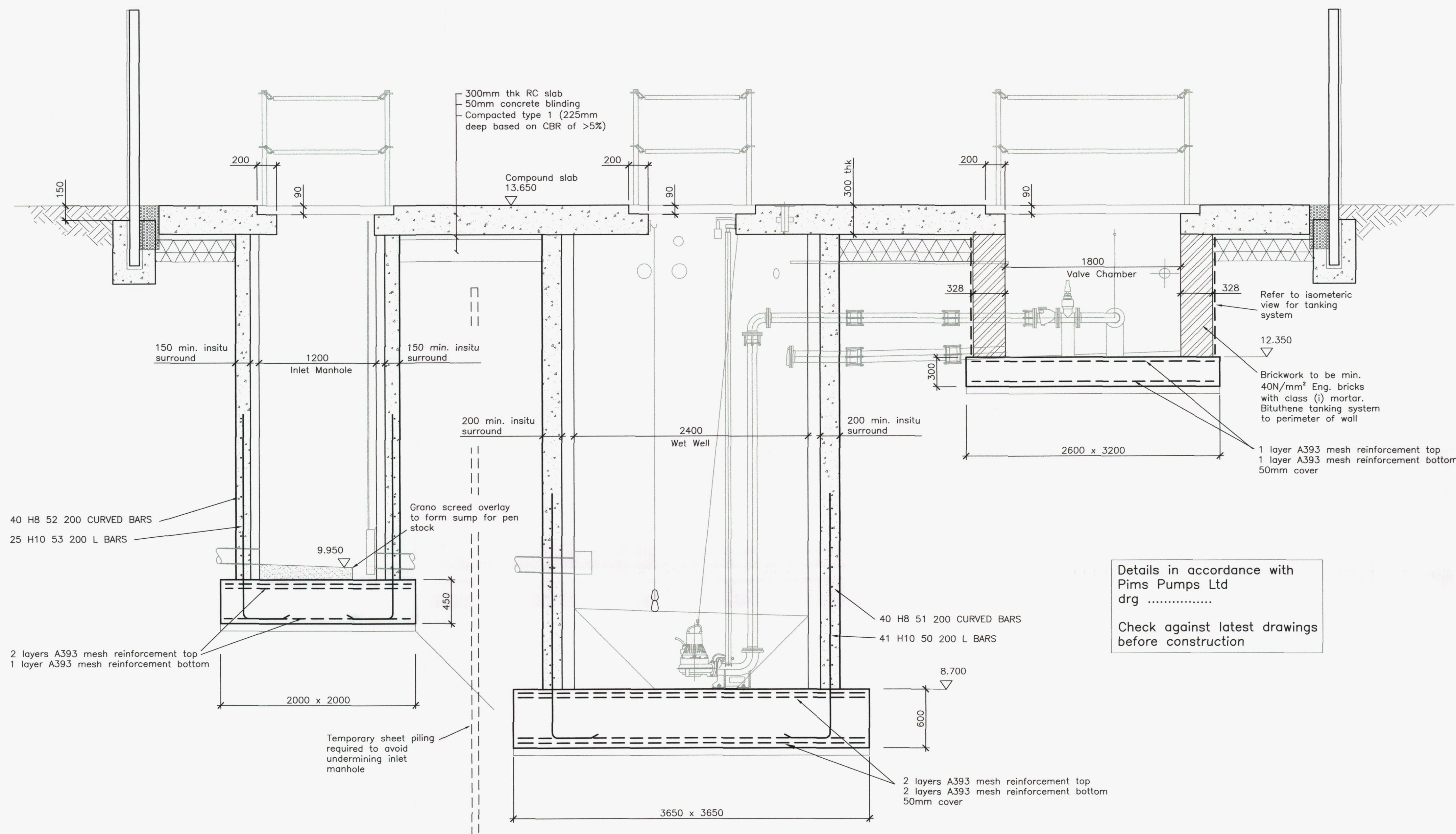
Section A - A (1:25)
