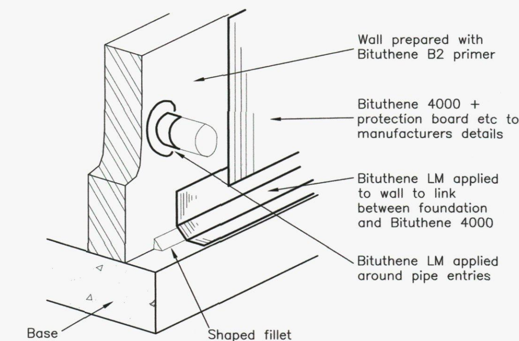
Isometric view on valve chamber wall
