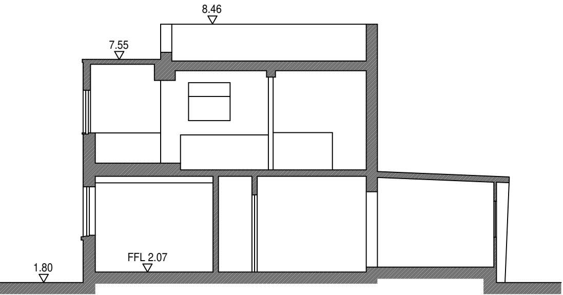
Existing Section
