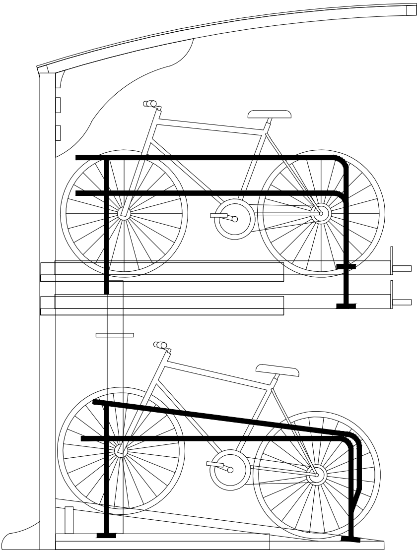
SIDE ELEVATION
