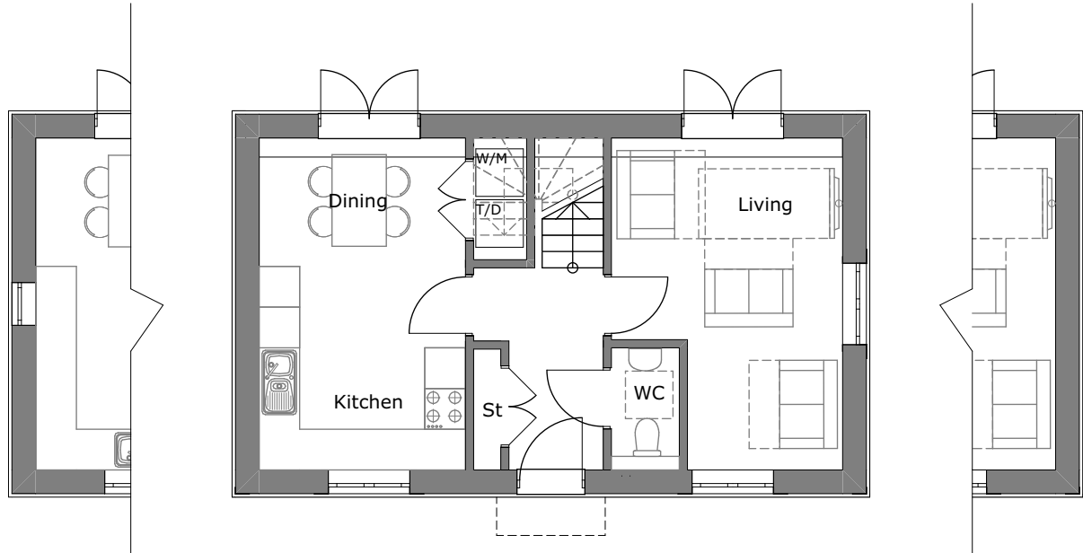
Ground Floor Plan to Plots 22 only
