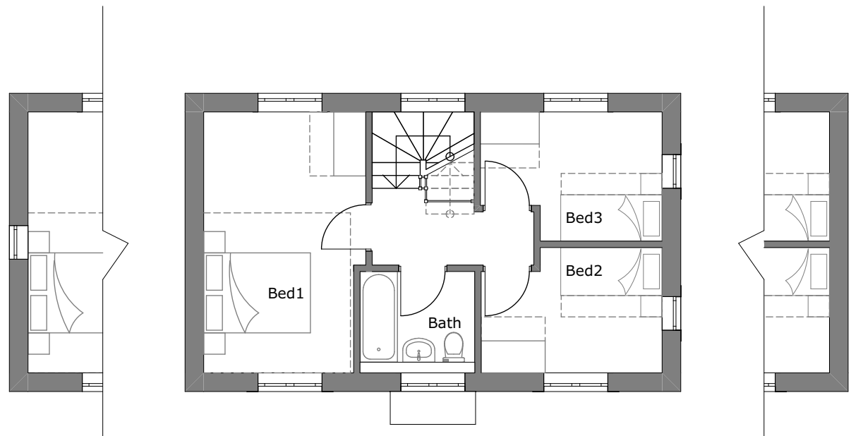
First Floor Plan to Plot 22 only
