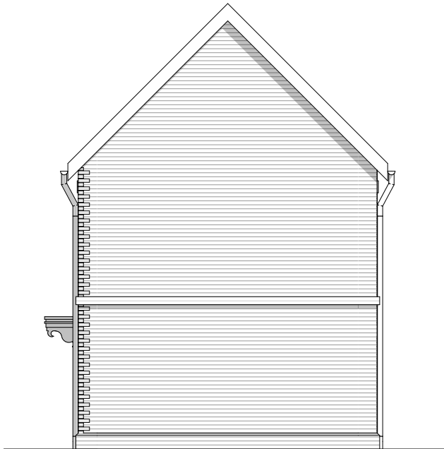
Side 1 Elevation to Plots 27&28
