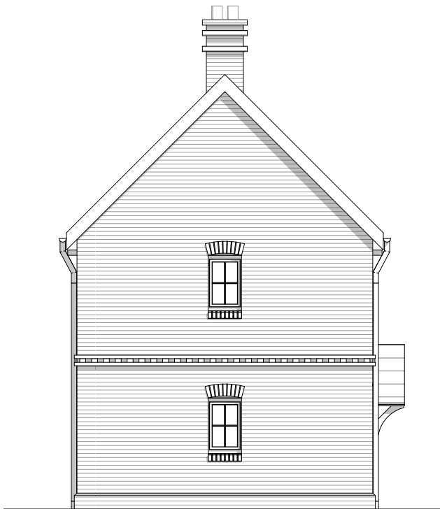
Side 2 Elevation to Plot 22
