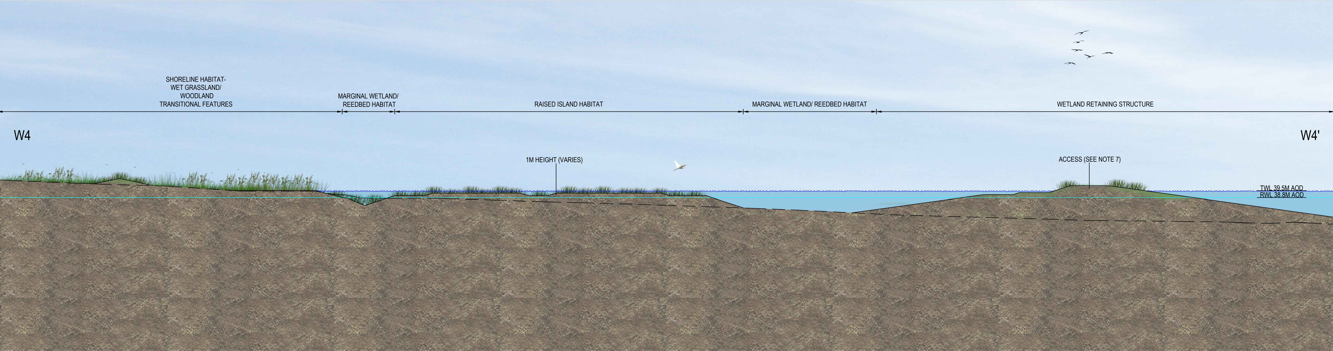
W4 - TYPICAL CROSS-SECTION THROUGH WETLAND ISLAND AND WETLAND RETAINING STRUCTURE SCALE 1:200
