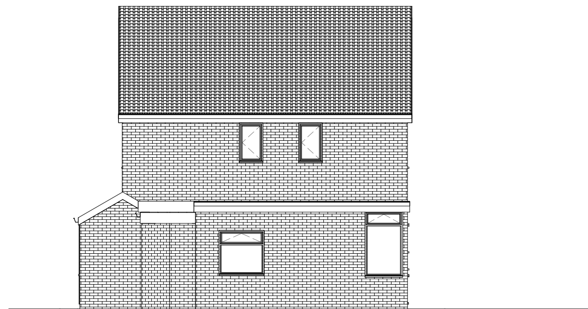
4 West Elevation 1 : 100
