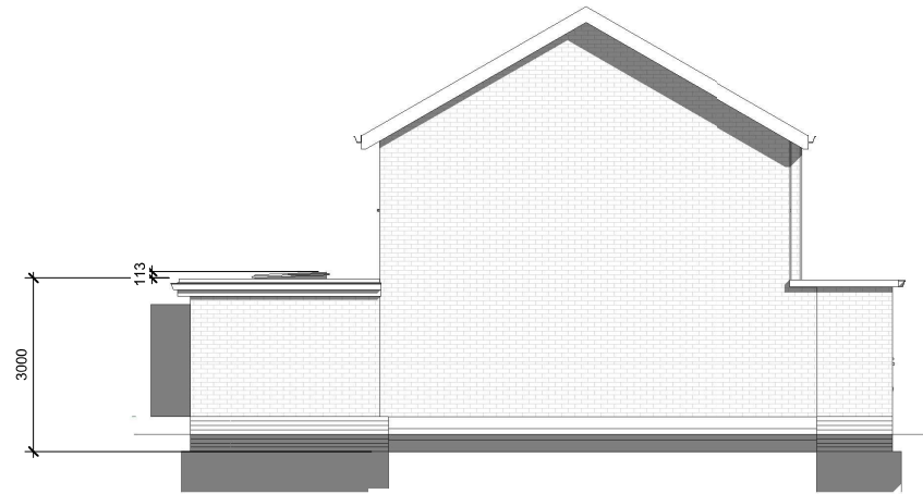
Proposed Elevation-Front
