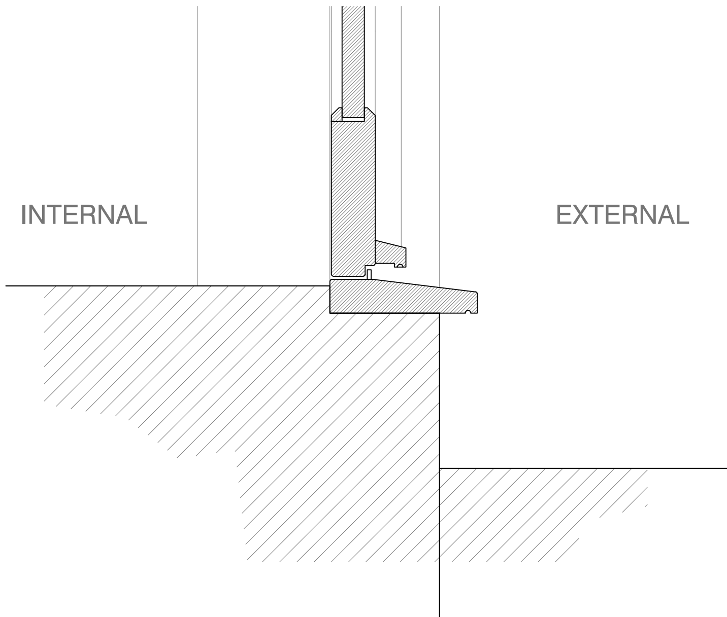
SECTION 1:5
