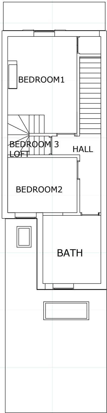
PROPOSED FIRST FLOOR PLAN
