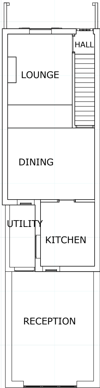
PROPOSED GROUND FLOOR PLAN
