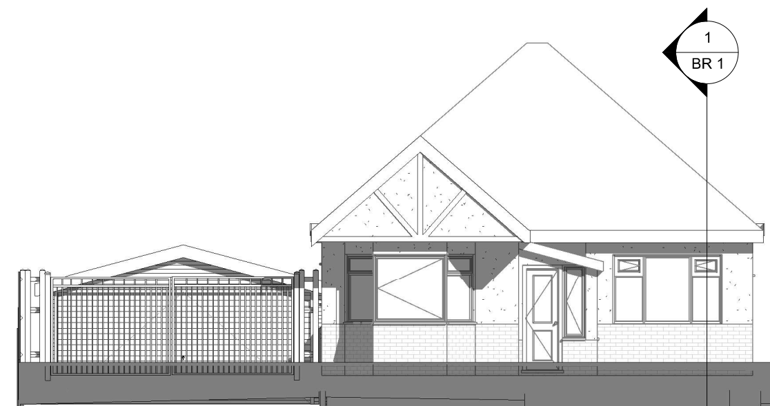
Proposed Elevation-Front
