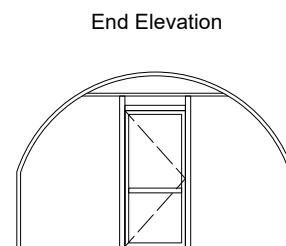
Polytunnel Elevations
