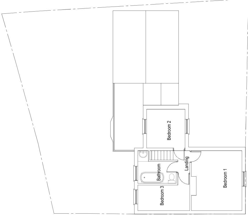
Existing First Floor Plan Scale 1:50
