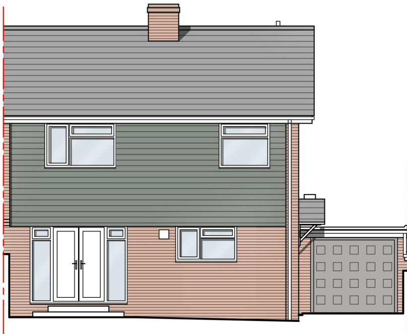
PROPOSED SOUTH WEST ELEVATION
