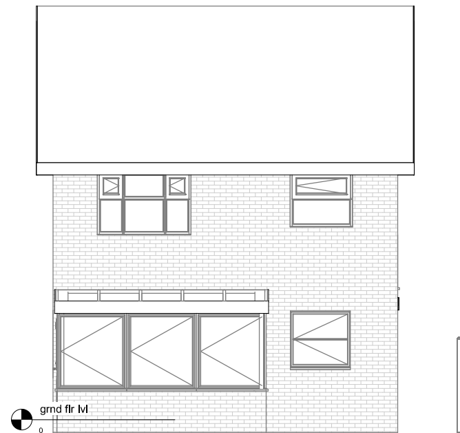
Existing Elevation-Rear
