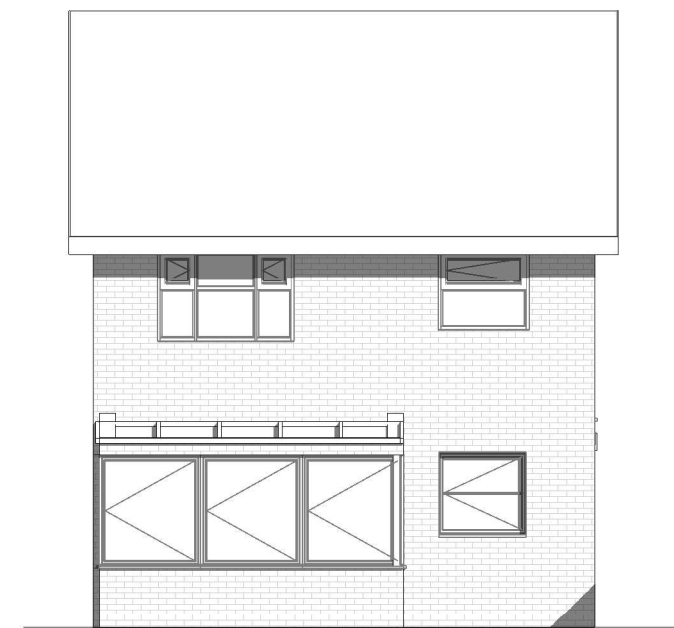
Proposed Elevation-Rear
