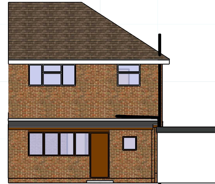
EXISTING SOUTH ELEVATION
