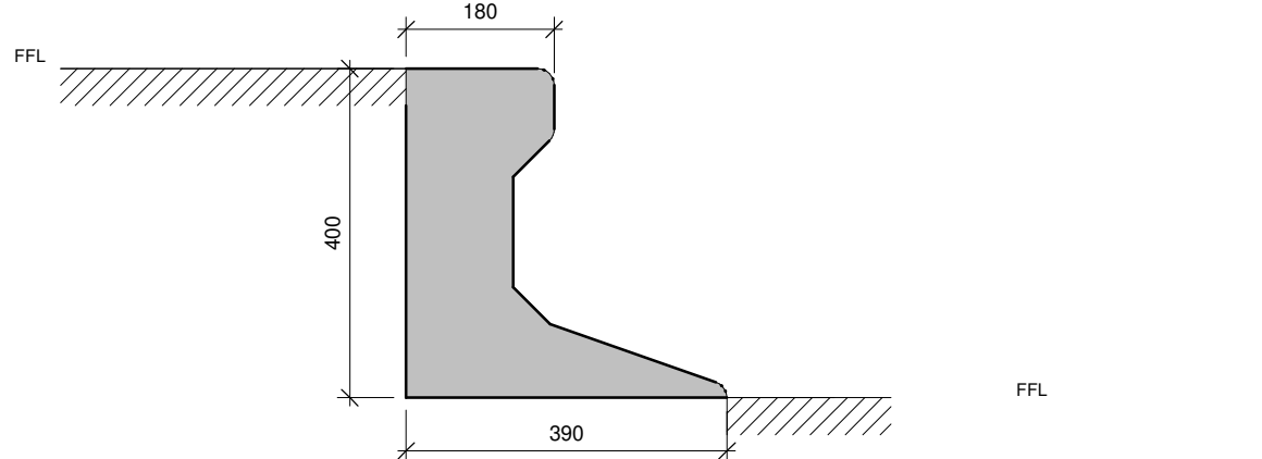
KT02 400 x 390mm PRECAST CONCRETE TRIEF KERB
