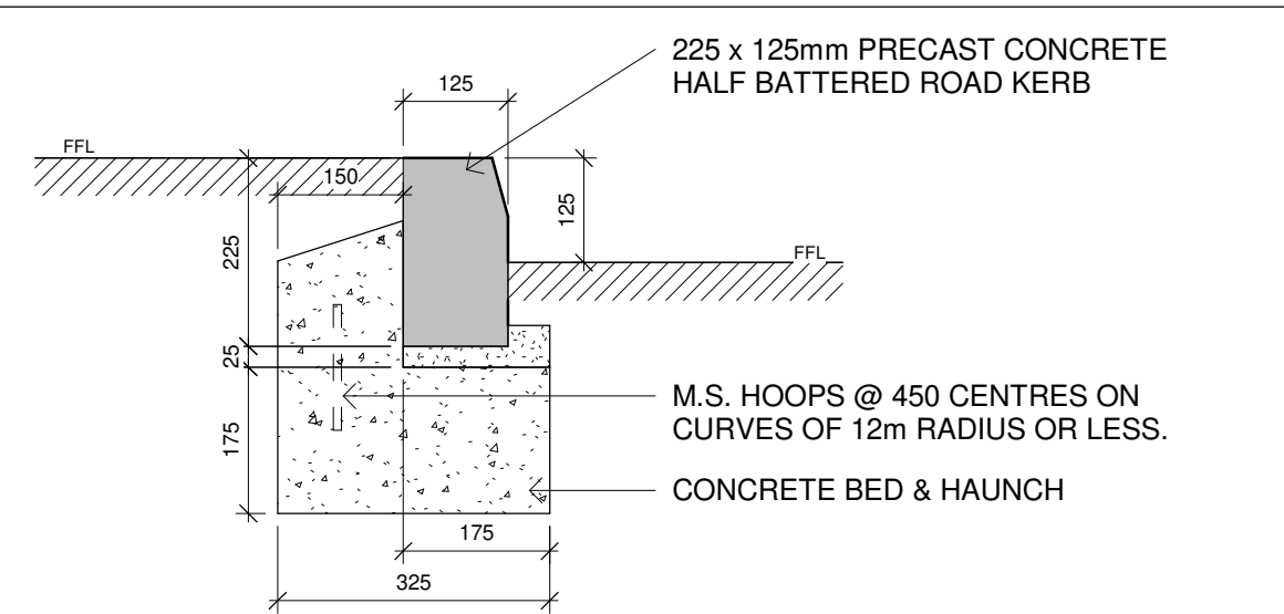
KT01 225 x 125mm PRECAST CONCRETE HALF BATTERED ROAD KERB
