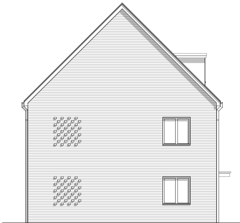
*Side Elevation
