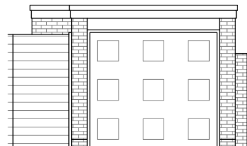
South Elevation 1:100
