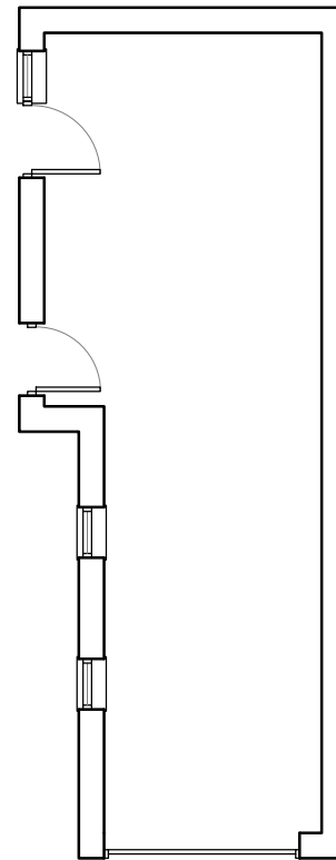
Ground Floor 1:100
