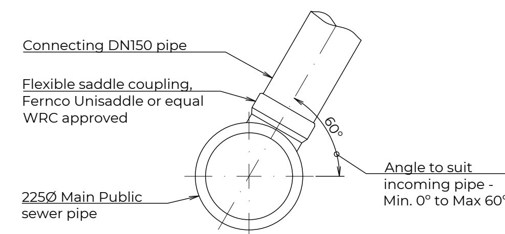
SECTION VIEW OF PUBLIC SEWER WITH CONNECTING PRIVATE PIPEWORK 1:10
