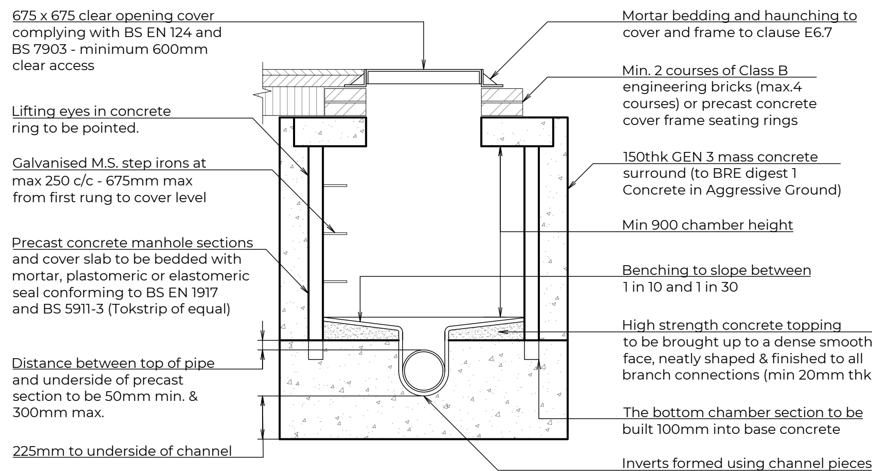
TYPE 2 MANHOLE - PC RINGS max depth 3.0m CL to pipe soffit 1:20
