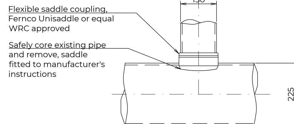
PUBLIC SEWER CONNECTION @ 90° 1:10
