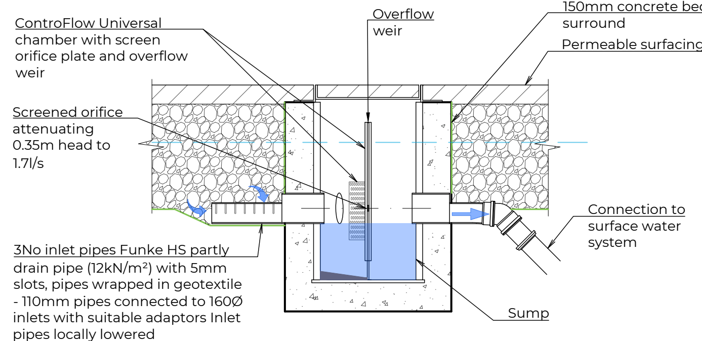
CONTROFLOW UNIVERSAL COLLECTION & ORIFICE CHAMBER - FC2 1:20
