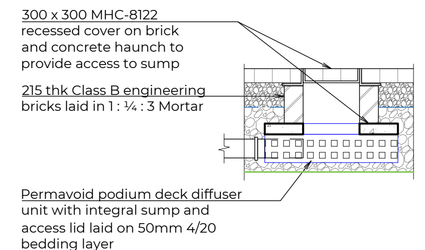
DIFFUSER UNIT WITH SUMP 1:20
