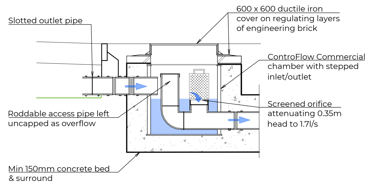
CONTROFLOW COMMERCIAL FLOW CONTROL CHAMBER - FC1 1:20
