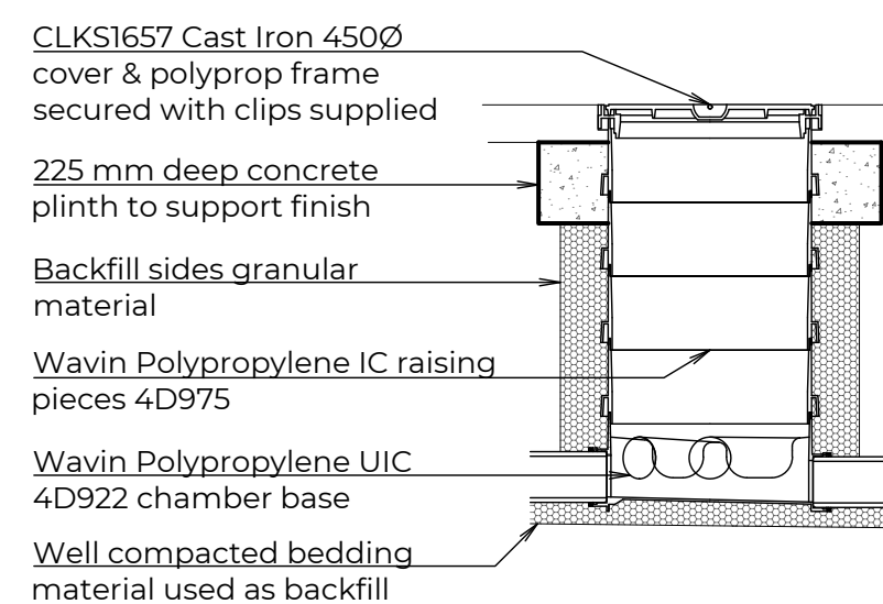
POLYPROPYLENE IC 450Ø IN PAVED LANDSCAPE 1:20
