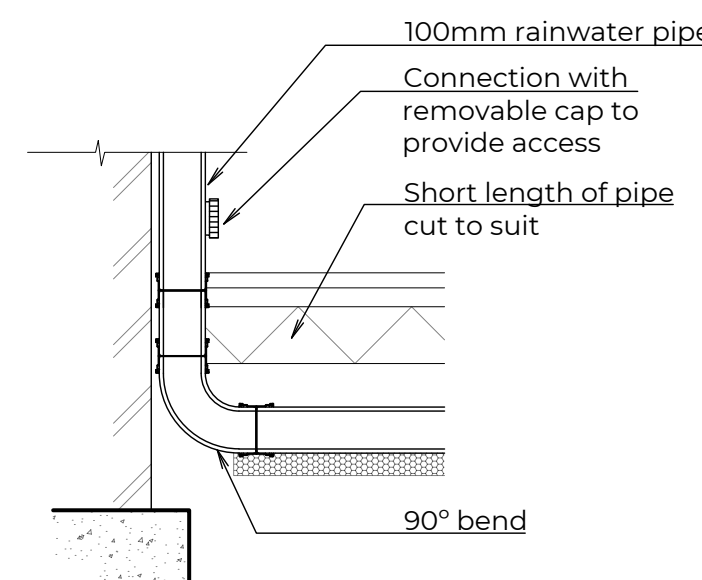
DOWN PIPE (100mm RODDABLE) 1:20
