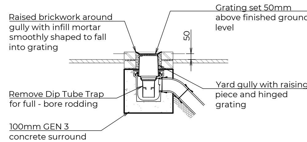
OVERFLOW GULLY DETAIL 1:20
