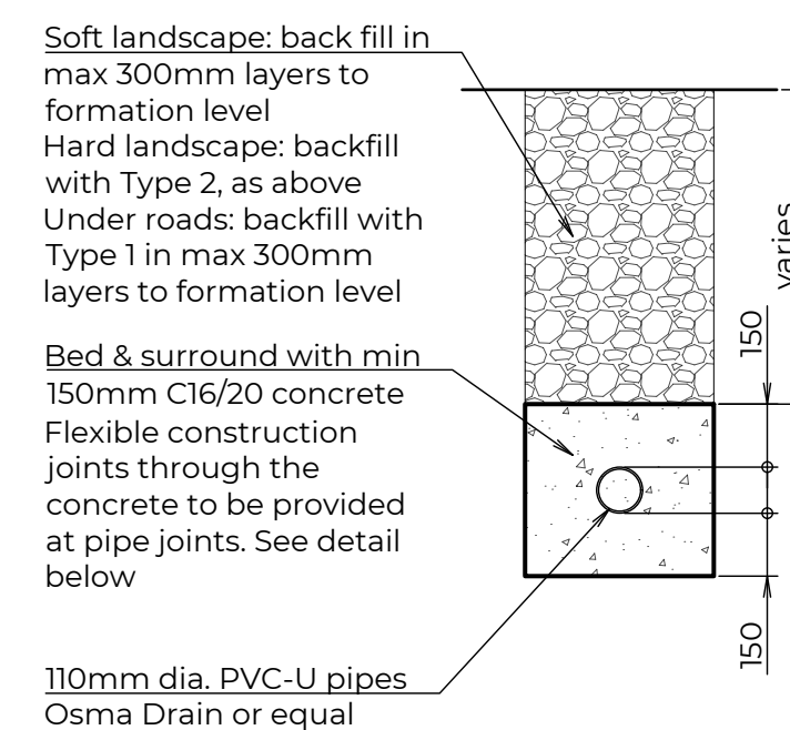
PRIVATE DRAINAGE - 110Ø CLASS Z BEDDING 1:20
