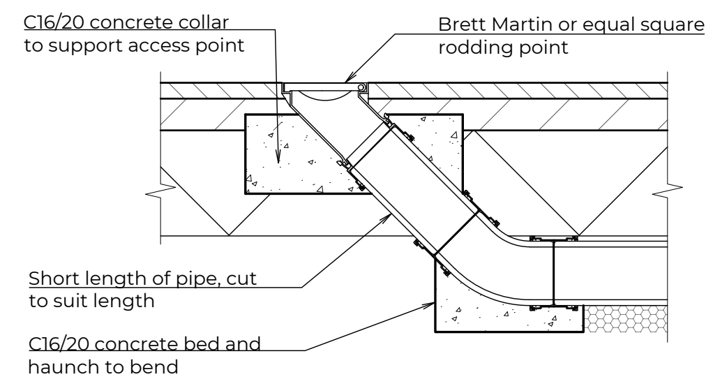
RODDING ACCESS IN HARD LANDSCAPE 1:10
