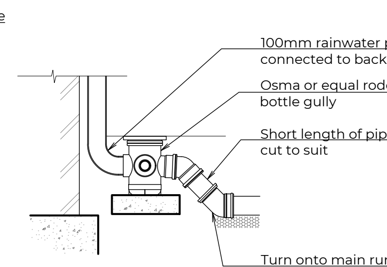
DOWN PIPE WITH GULLY (100mm RODDABLE) 1:20
