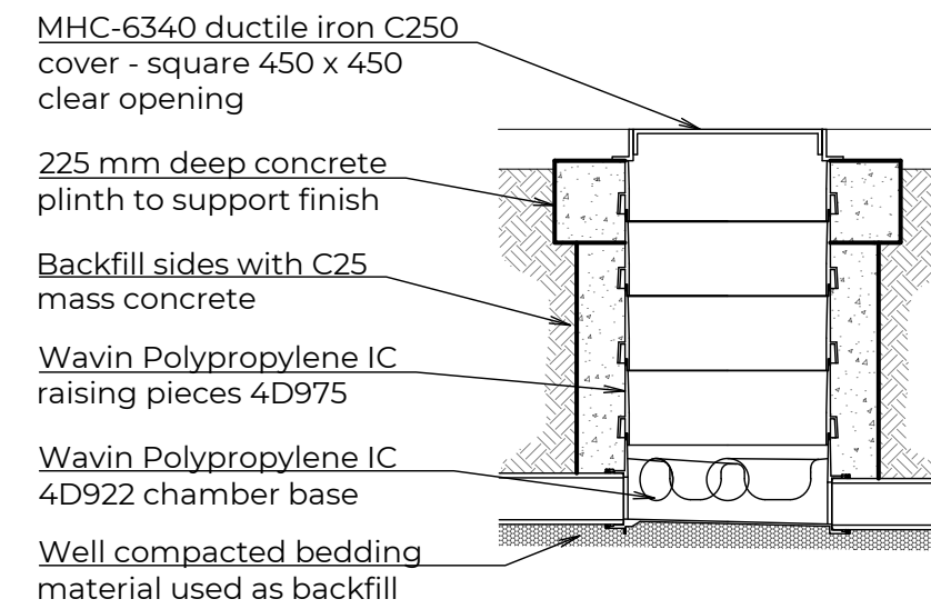
POLYPROPYLENE IC 450Ø - C250 IRON COVER ADJACENT ROADS 1:20
