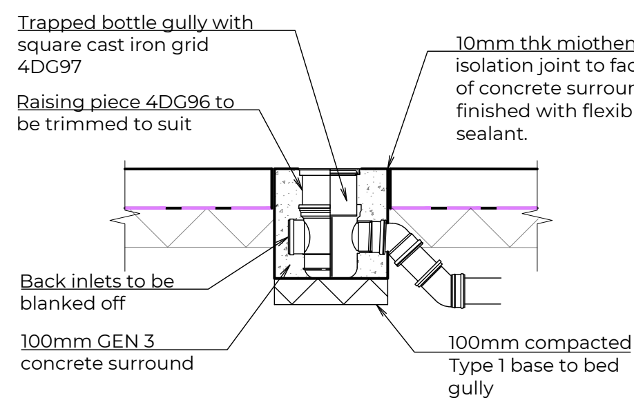
TRAPPED GULLY IN BIN SLAB 1:20
