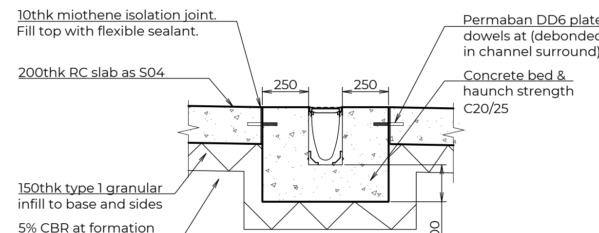
ACO MULTIDRAIN M100D 10.0 CHANNEL 1:20
