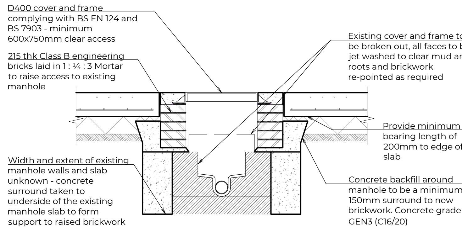
RAISED MANHOLE DETAIL 1:20
