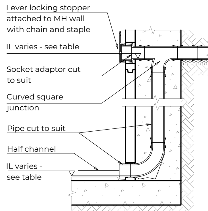
BACKDROP CONNECTION TO MANHOLE 1:20
