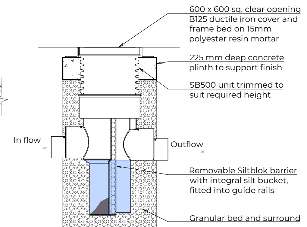
TURTLE ENVIRO SILT BLOK 500 SILT TRAP 1:20
