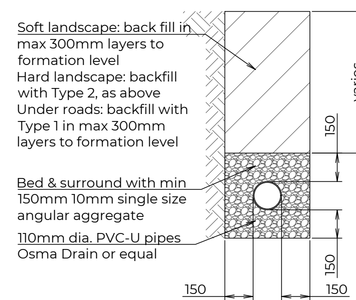
PRIVATE DRAINAGE - 110Ø CLASS S BEDDING 1:20
