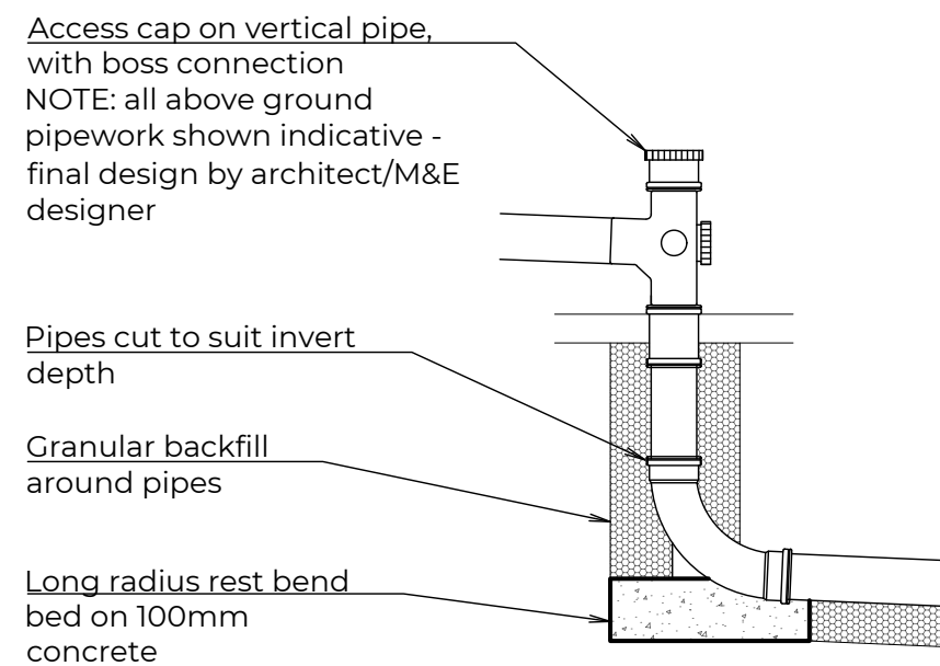
EXTERNAL STUB STACK CONNECTION 1:20
