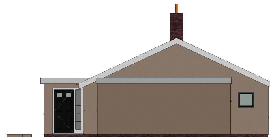
4 West Elevation 1 : 100
