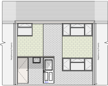
EXISTING FRONT ELEVATION - A Scale 1:50
