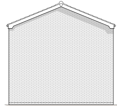
EXISTING SIDE ELEVATION - C Scale 1:50
