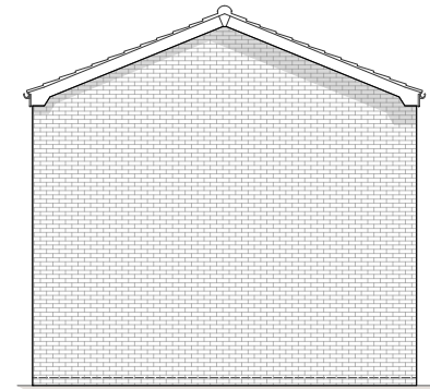
PROPOSED SIDE ELEVATION - C Scale 1:50
